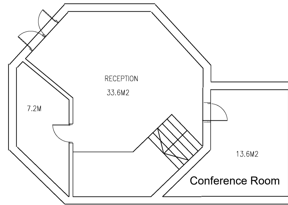
GROUND FLOOR PLAN VIEW
