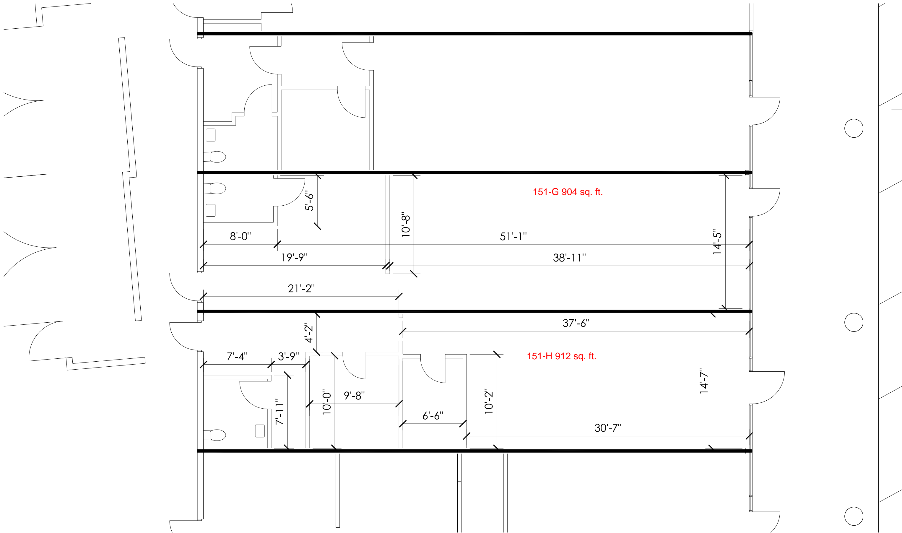
151-G & 151-H, INTERIOR DIMENSIONS GRASS VALLEY, CA
