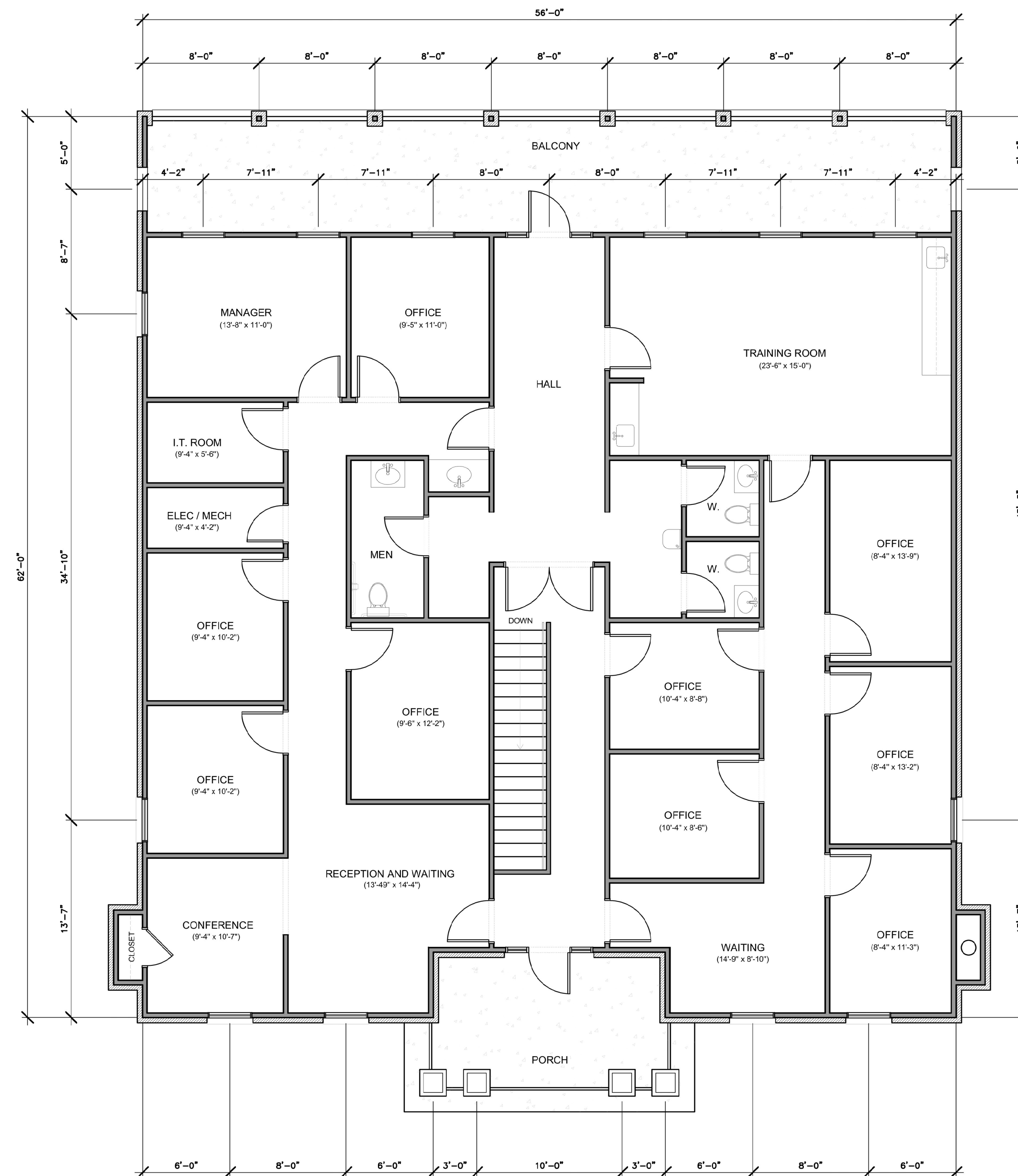
SECOND FLOOR PLAN (AS BUILT) SCALE: 3/16" = 1'-0"
