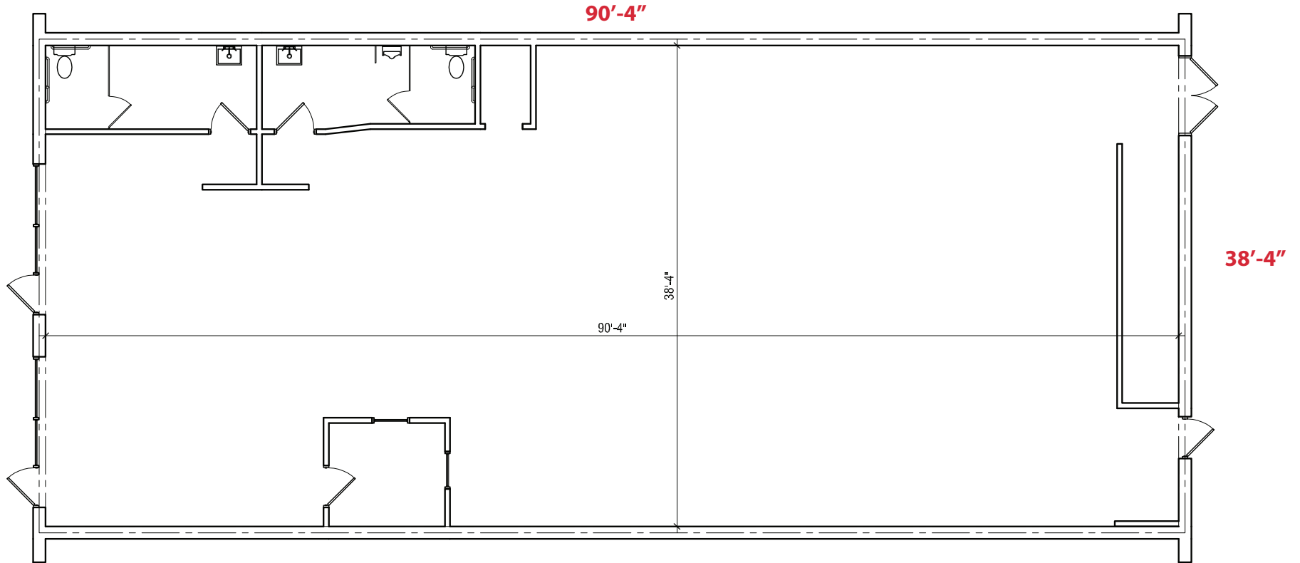
1 FLOOR PLAN - 771 1/4" = 1'-0"
