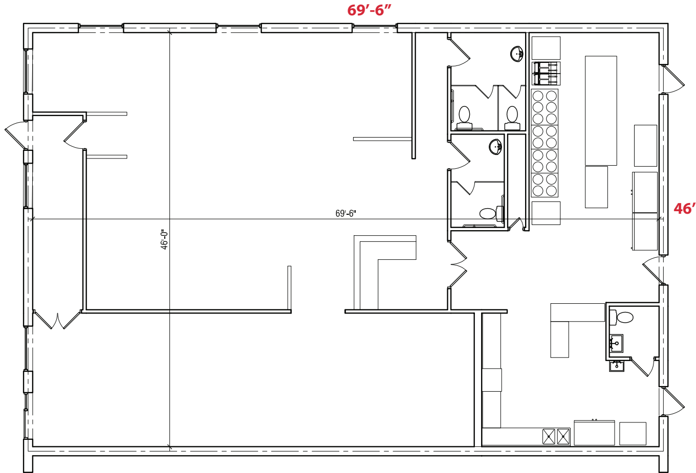
1 FLOOR PLAN - 771 1/8" = 1'-0"
