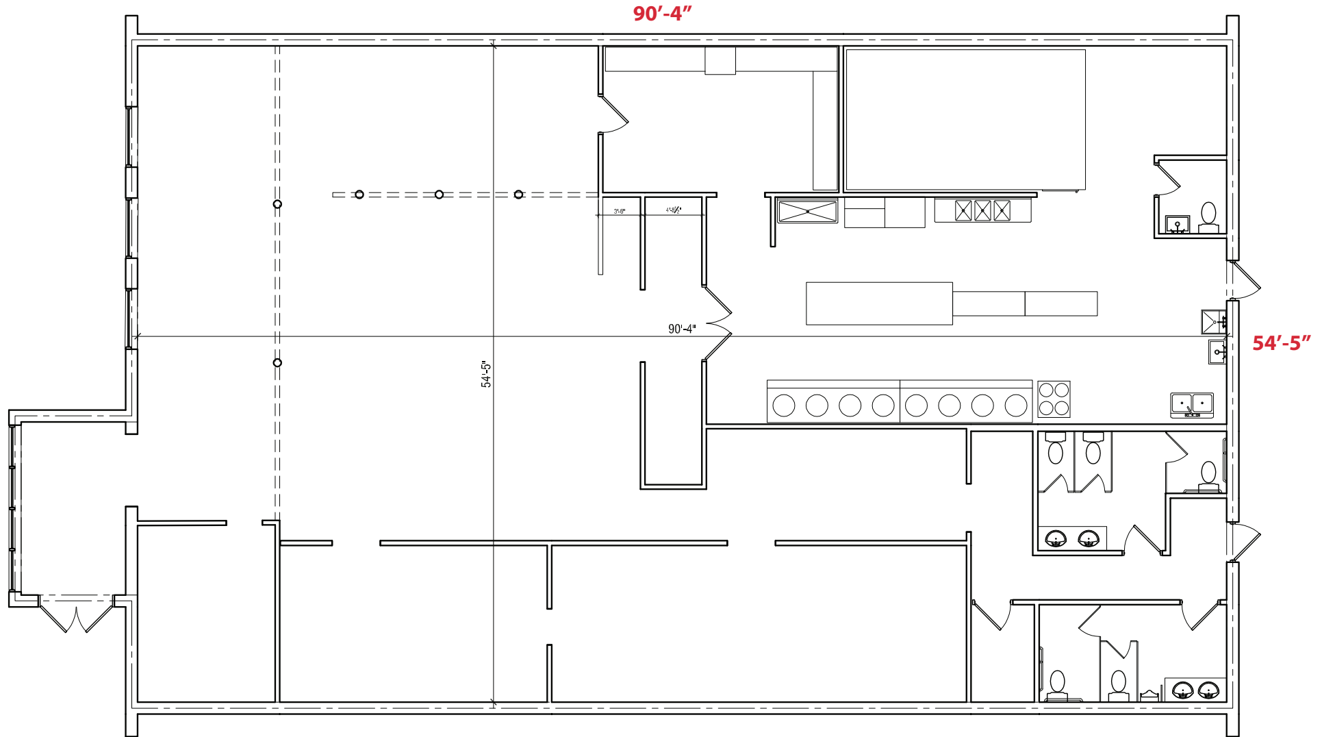
1 FLOOR PLAN - 781 1/4" = 1'-0"
