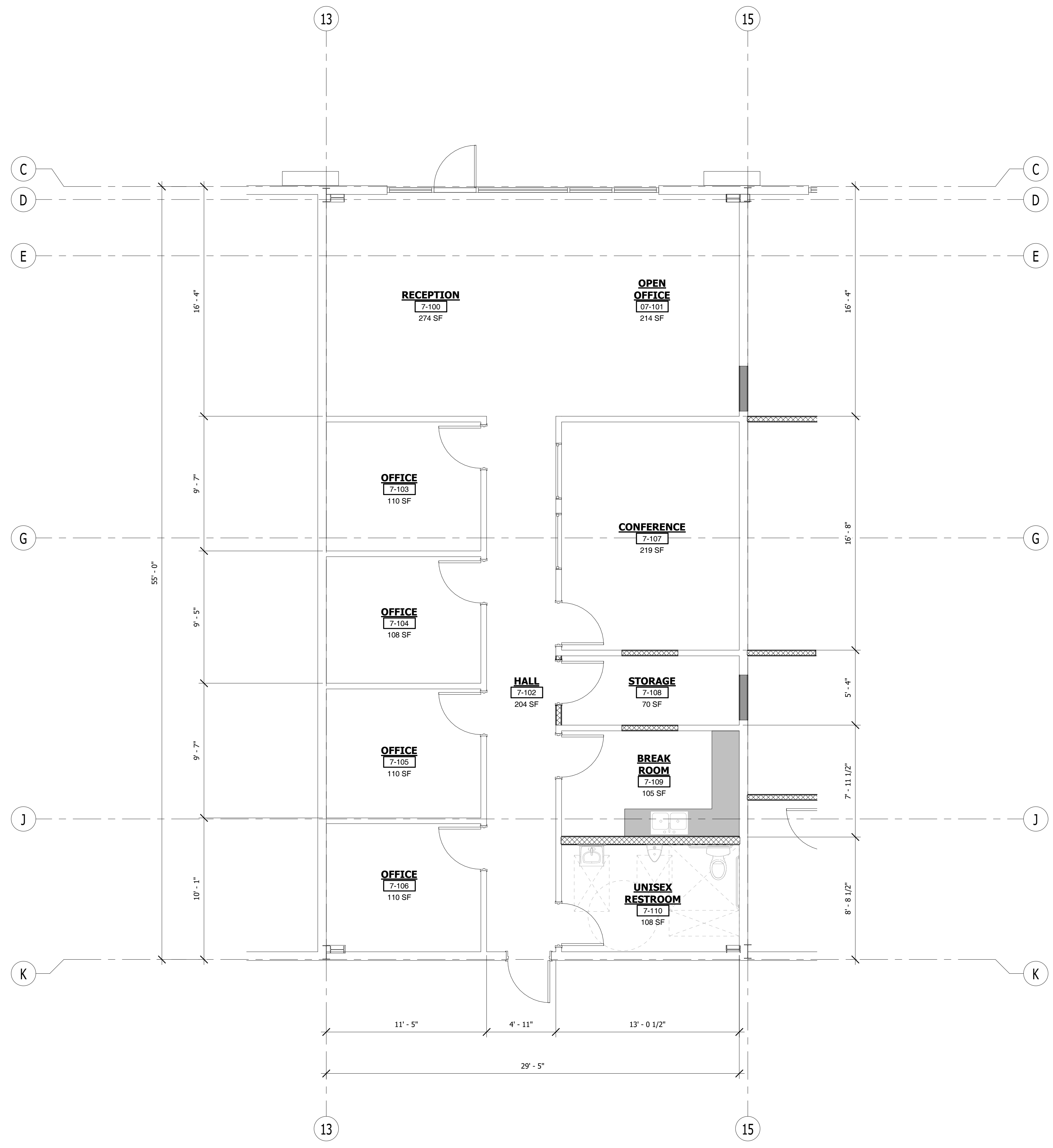
1 ENLARGED FLOOR PLAN -- SUITE 7
