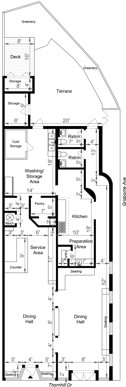
FLOOR PLAN
