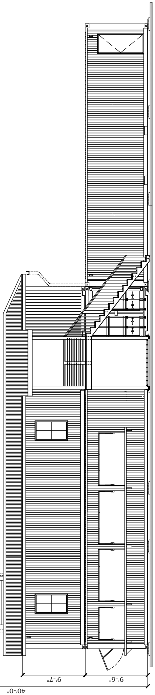
ELEVATION 2 1/4" = 1'-0"
