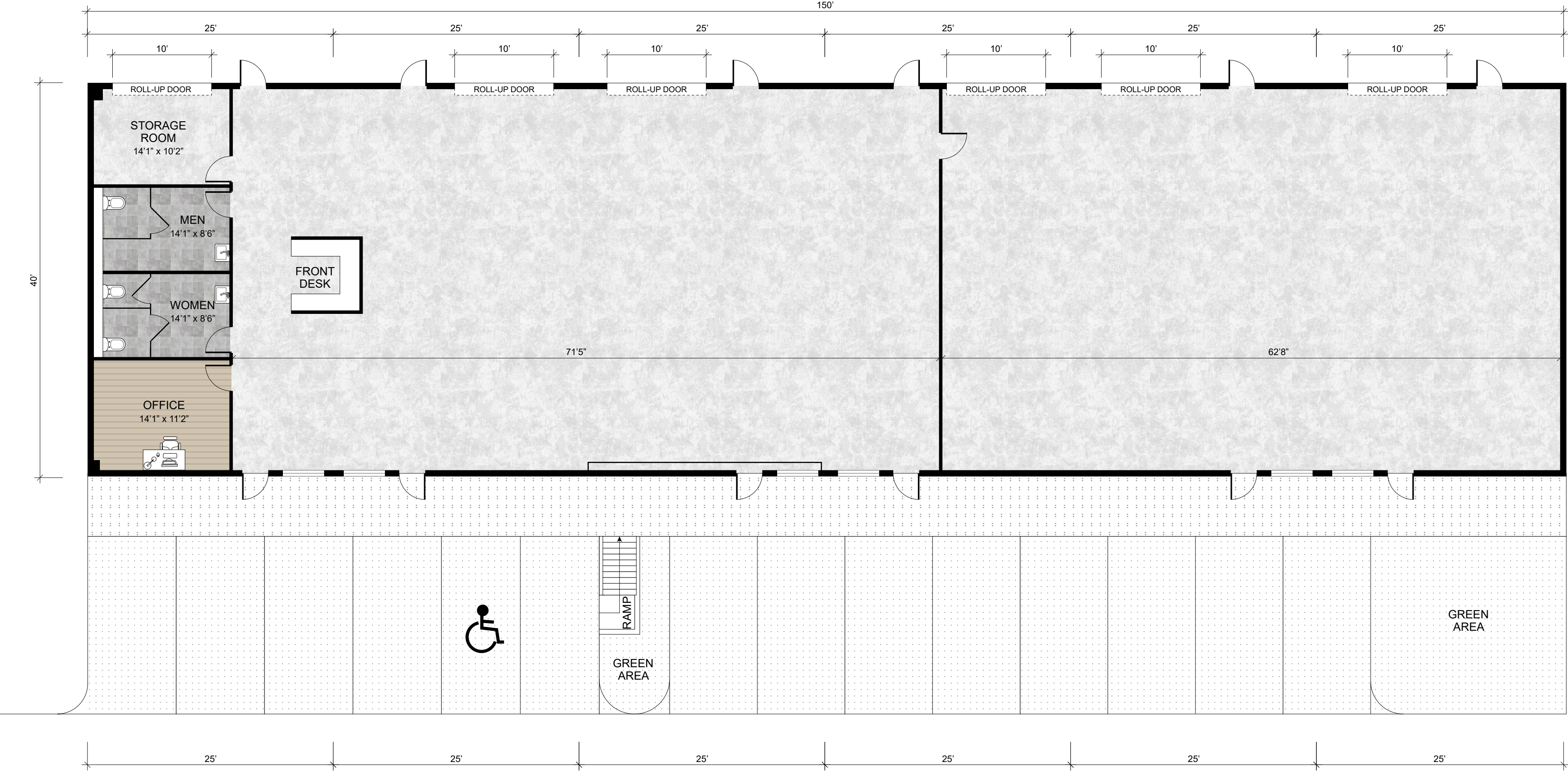
FLOOR PLAN BLDG. 331
