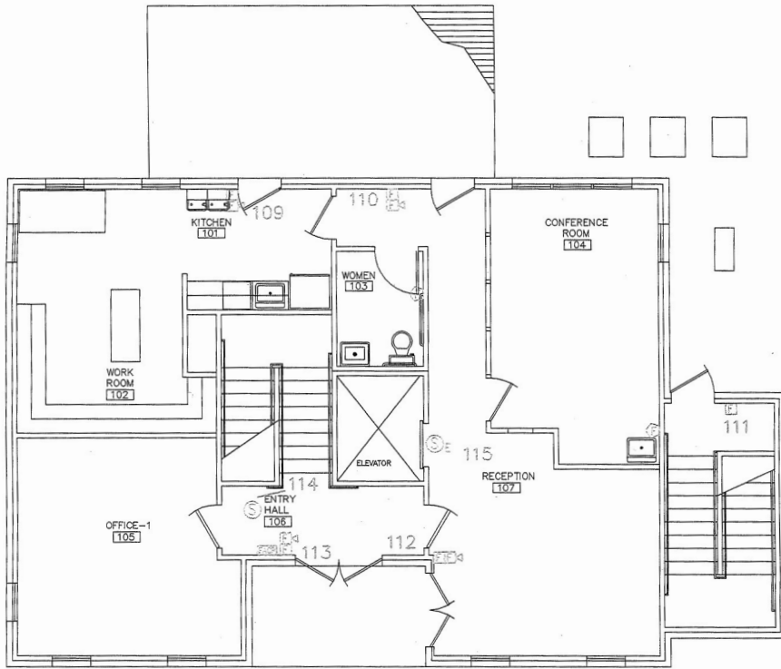
First Level Plan
