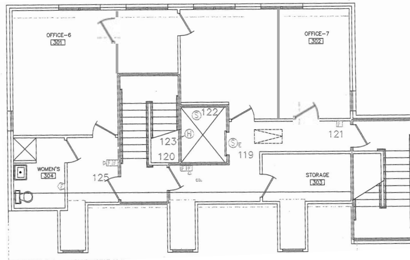
Third Level Plan
