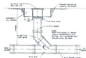
TYPICAL CLEAN OUT DETAIL
