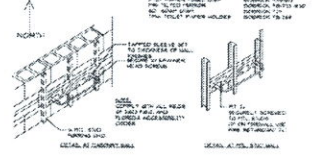
GRAB BAR INSTALLATION DETAIL
