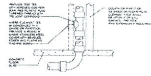
TYPICAL WALL CLEAN OUT DETAIL
