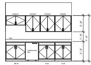
4 KITCHEN #38 - ELEVATION 3/8" = 1'-0"
