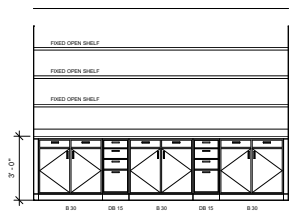
6 COPY #29 ELEVATION 3/8" = 1'-0"
