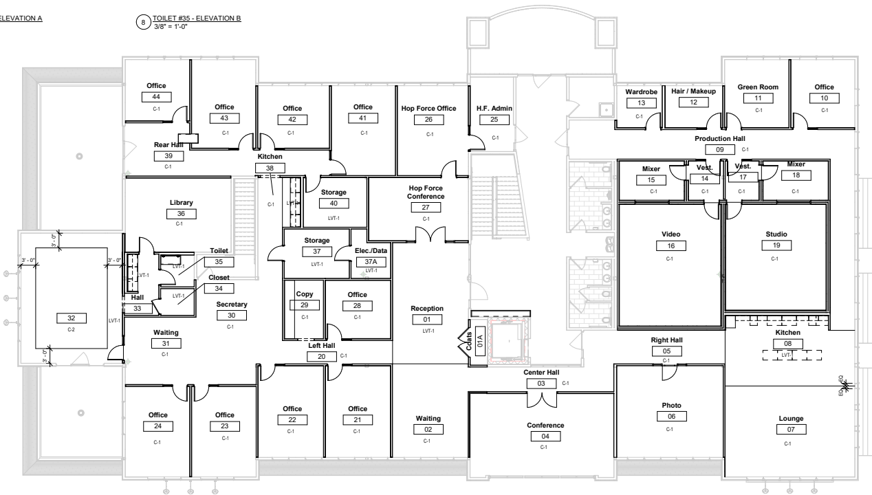
1 SECOND FLOOR FINISH PLAN 1/8" = 1'-0"
