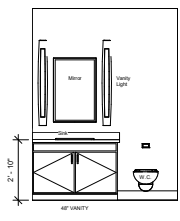
7 TOILET #35 - ELEVATION A 3/8" = 1'-0"
