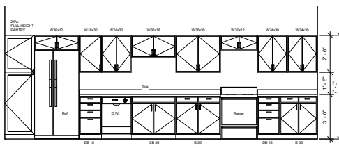
2 KITCHEN #08 - ELEVATION A 3/8" = 1'-0"
