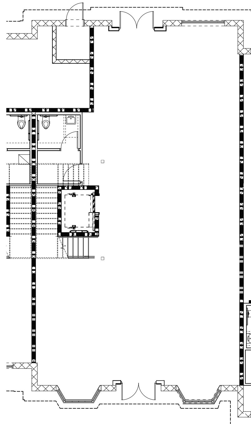
FIRST FLOOR
