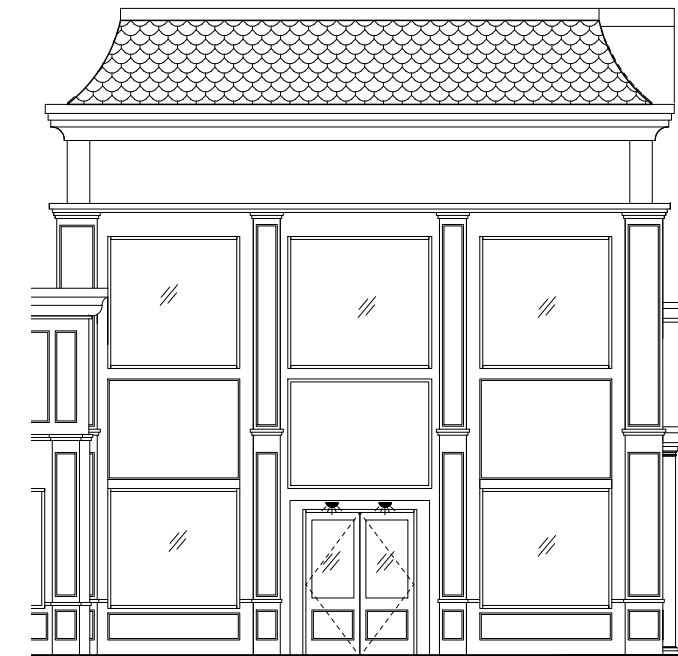
COURTYARD ELEVATION
