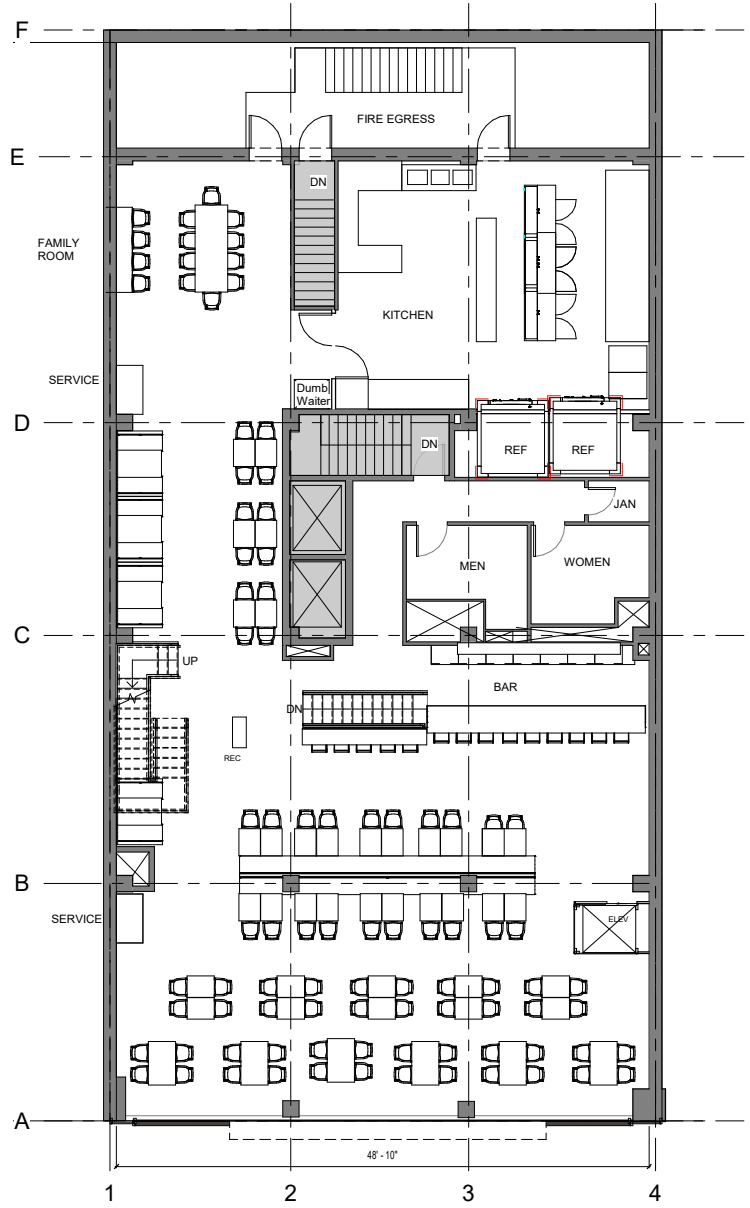
① 2ND FLOOR With Third 1/8" = 1'-0"
