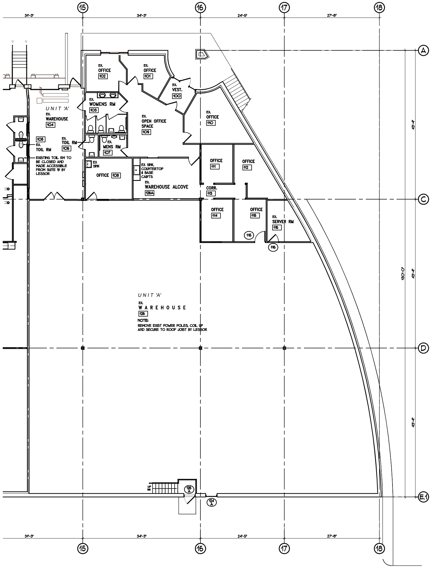
FLOOR PLAN SCALE: 1/16" = 1'-0"
