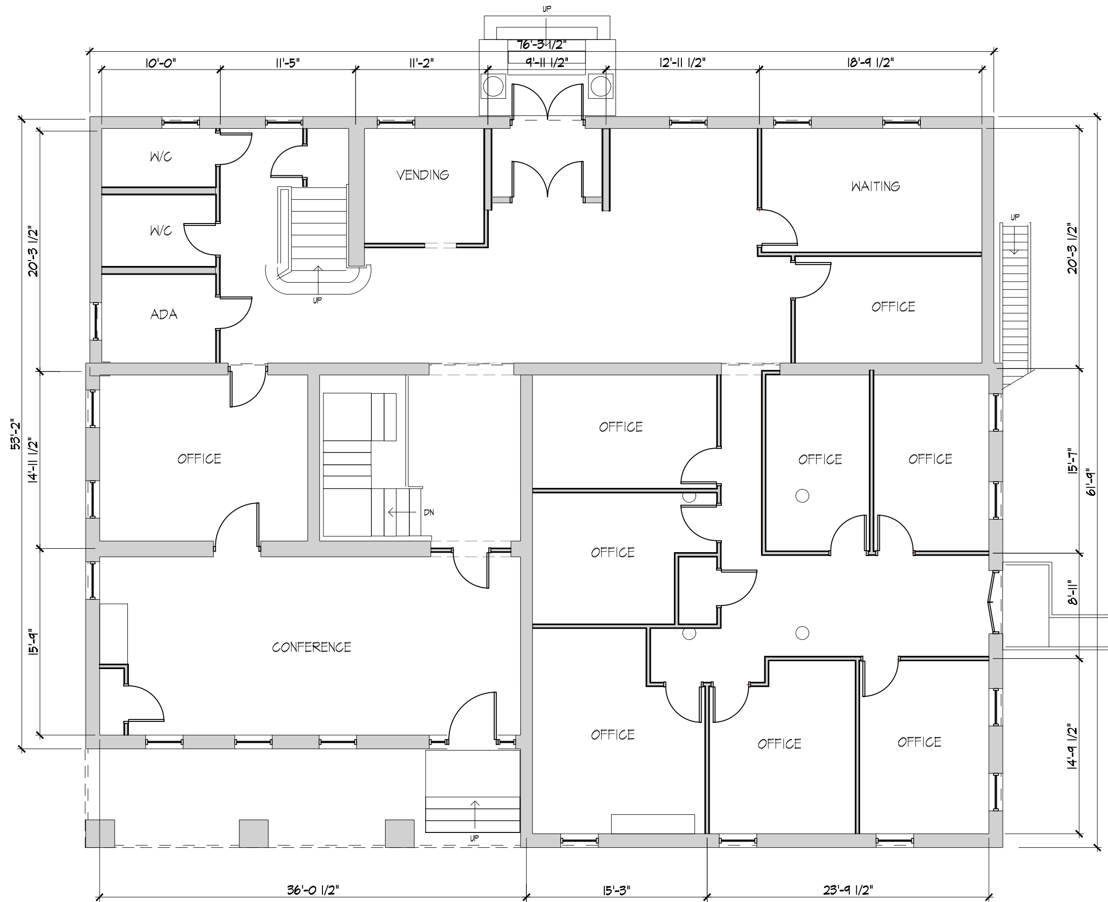
FIRST FLOOR PLAN 7 CLAYTON AVENUE
