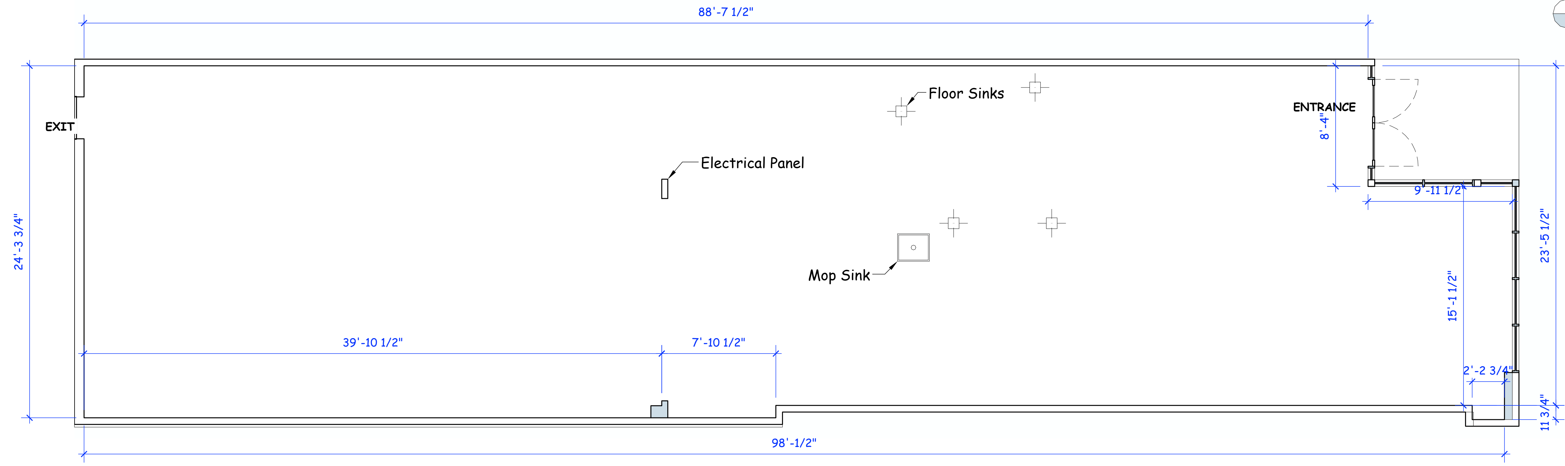
Measured Floorplan 1/4" = 1'-0"
