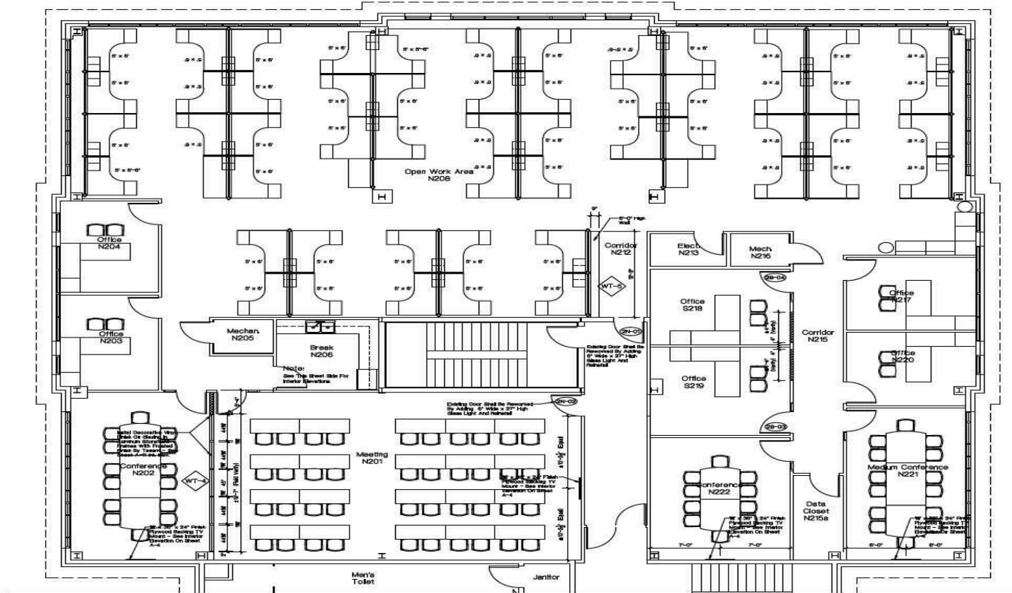
Partial Second Floor Plan North - Renovation 1/8" = 1'-0"
