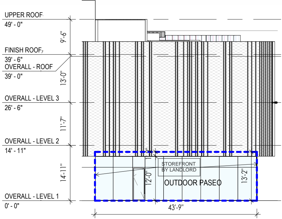
3 PASEO ELEVATION - RETAIL R16 LOD SCALE: 1/16" = 1'-0"
