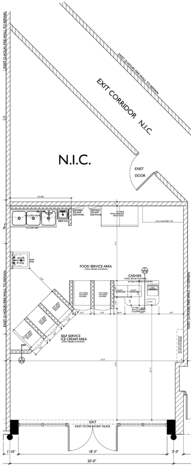
ICE CREAM SHOP 580 S.Q. FT.
