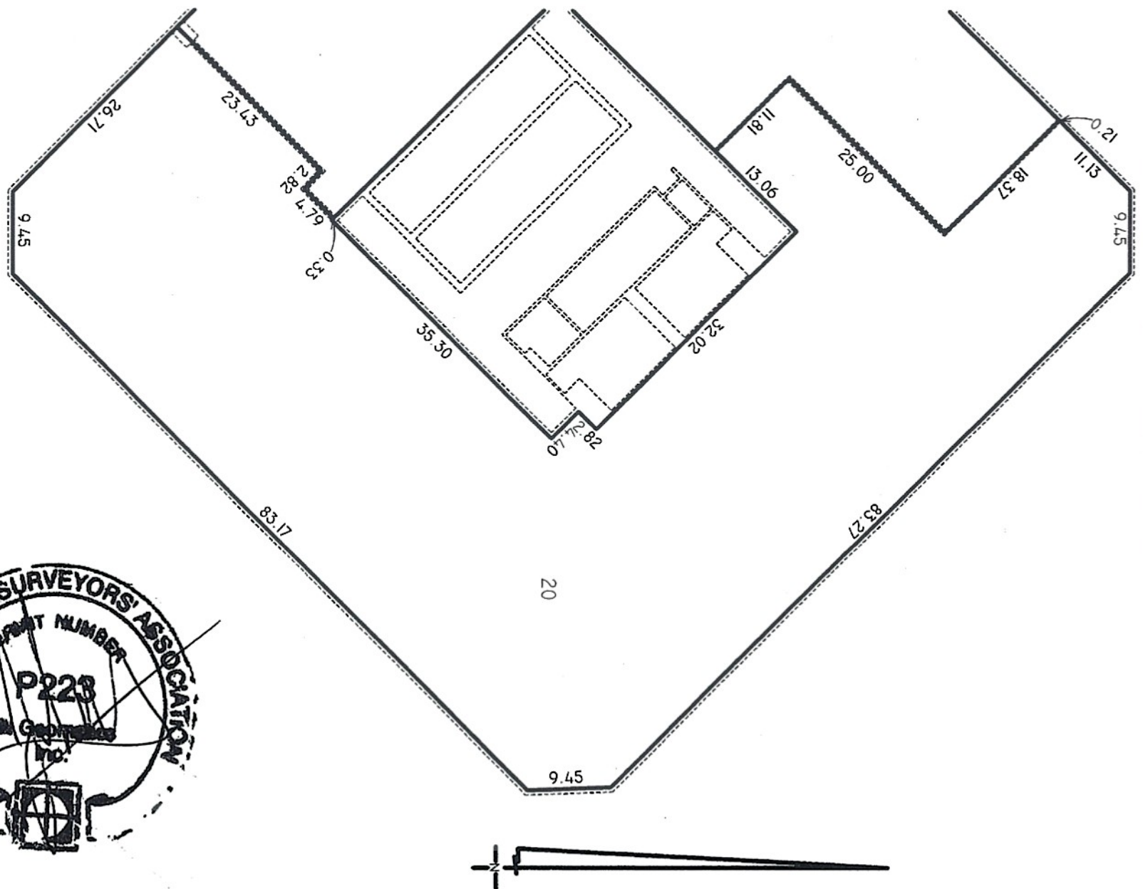
UNIT 20 NOT TO SCALE
