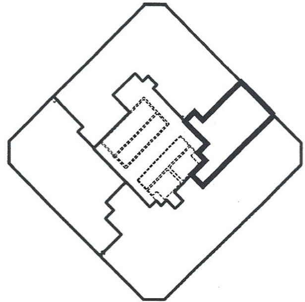
NINTH FLOOR PLAN UNIT 33 NOT TO SCALE
