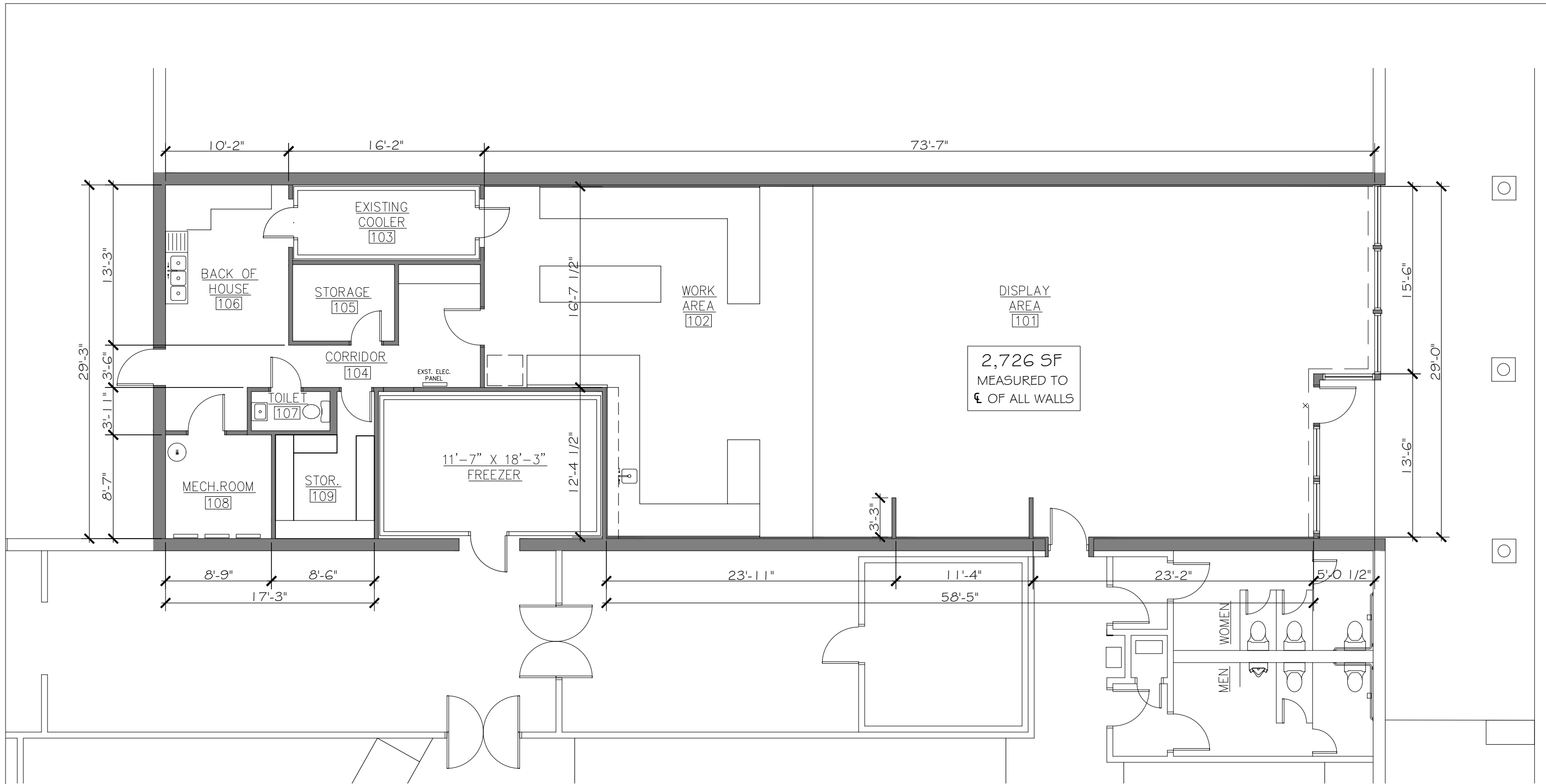
1 FLOOR PLAN A1.0 SCALE: 1/8" = 1'-0" 0 5' 10'
