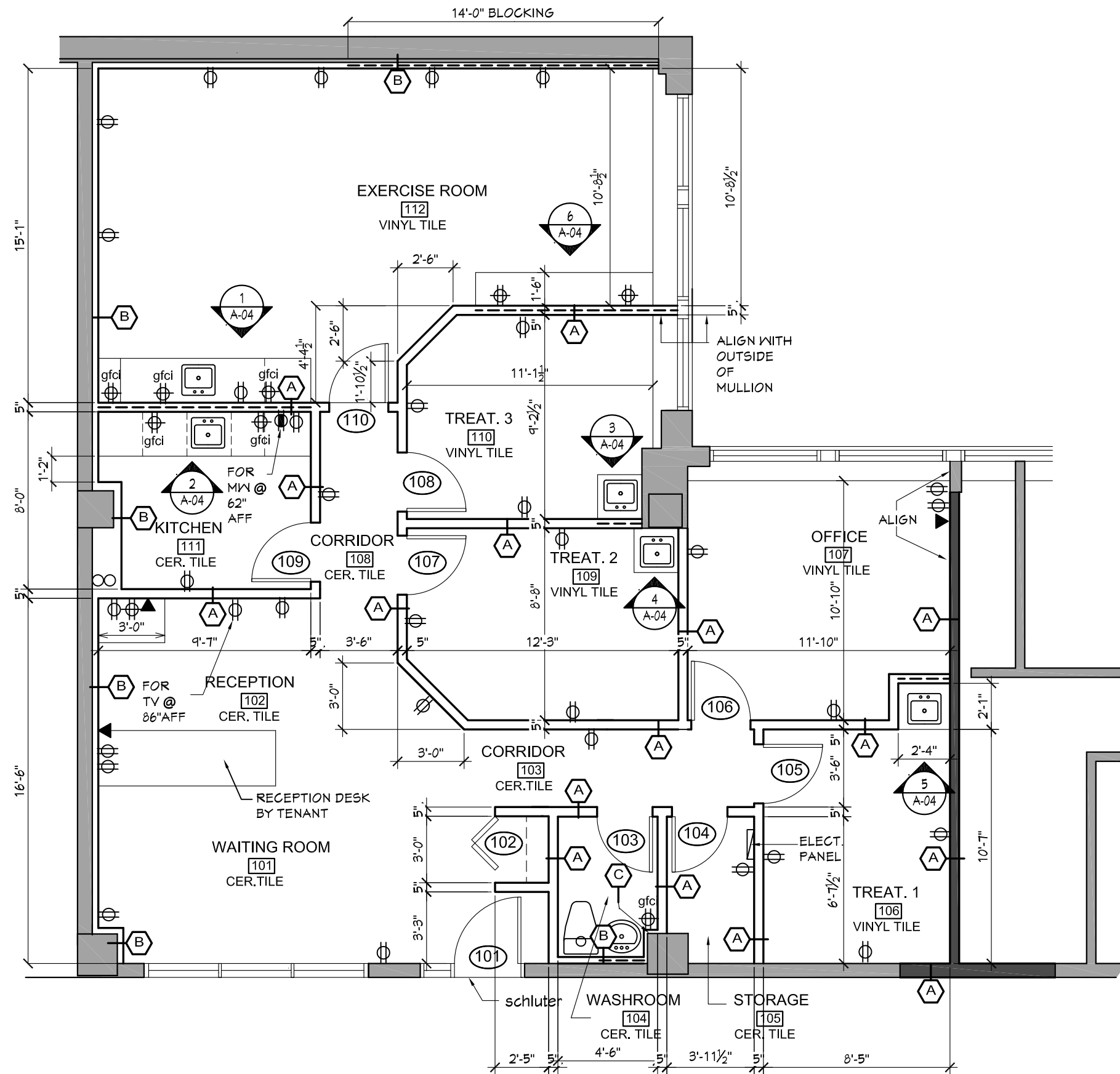
1 FLOOR PLAN A-02 3/16" = 1'-0"
