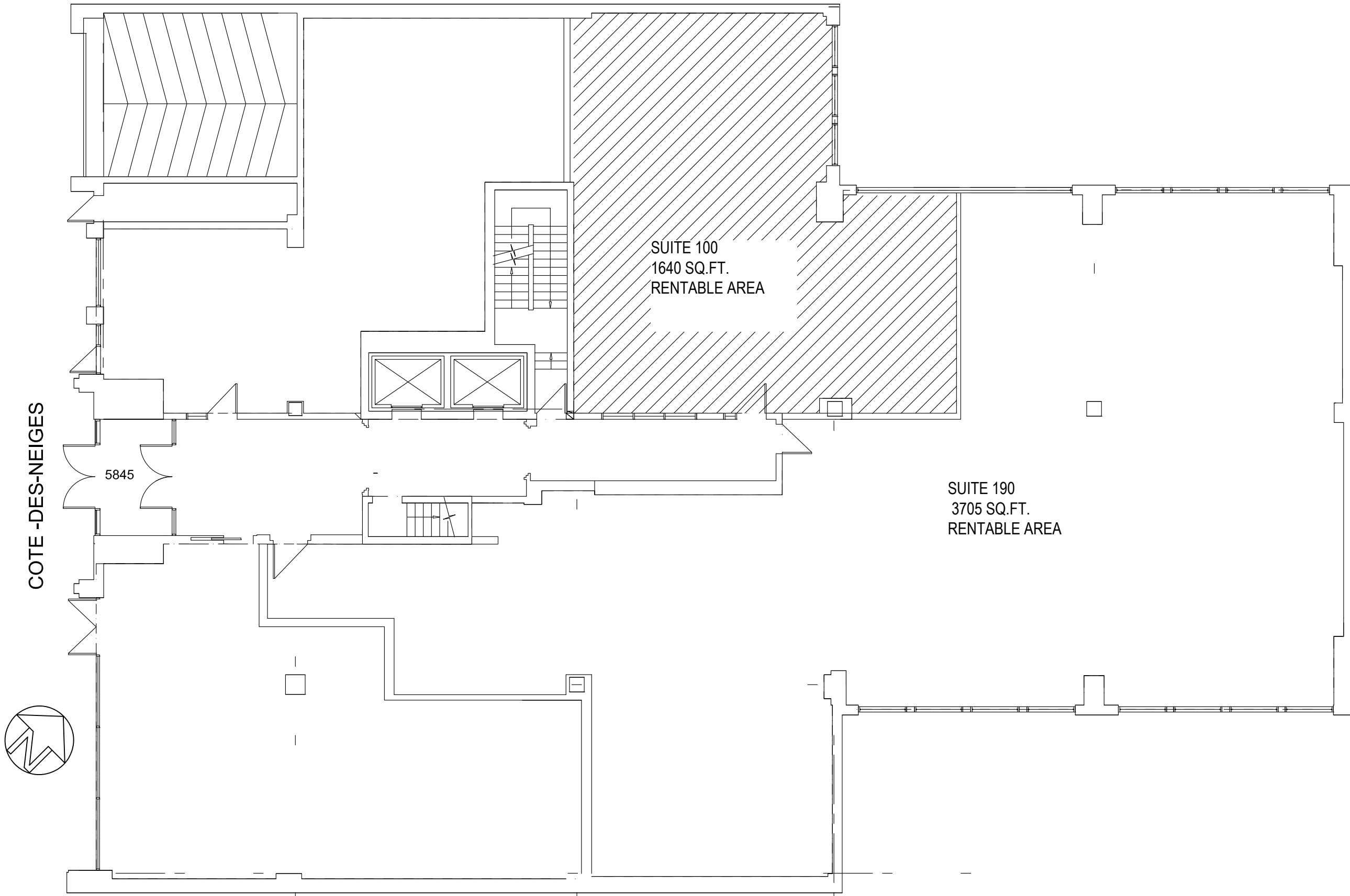
1 GROUND FLOOR KEY PLAN A-01 1" = 10'-0"
