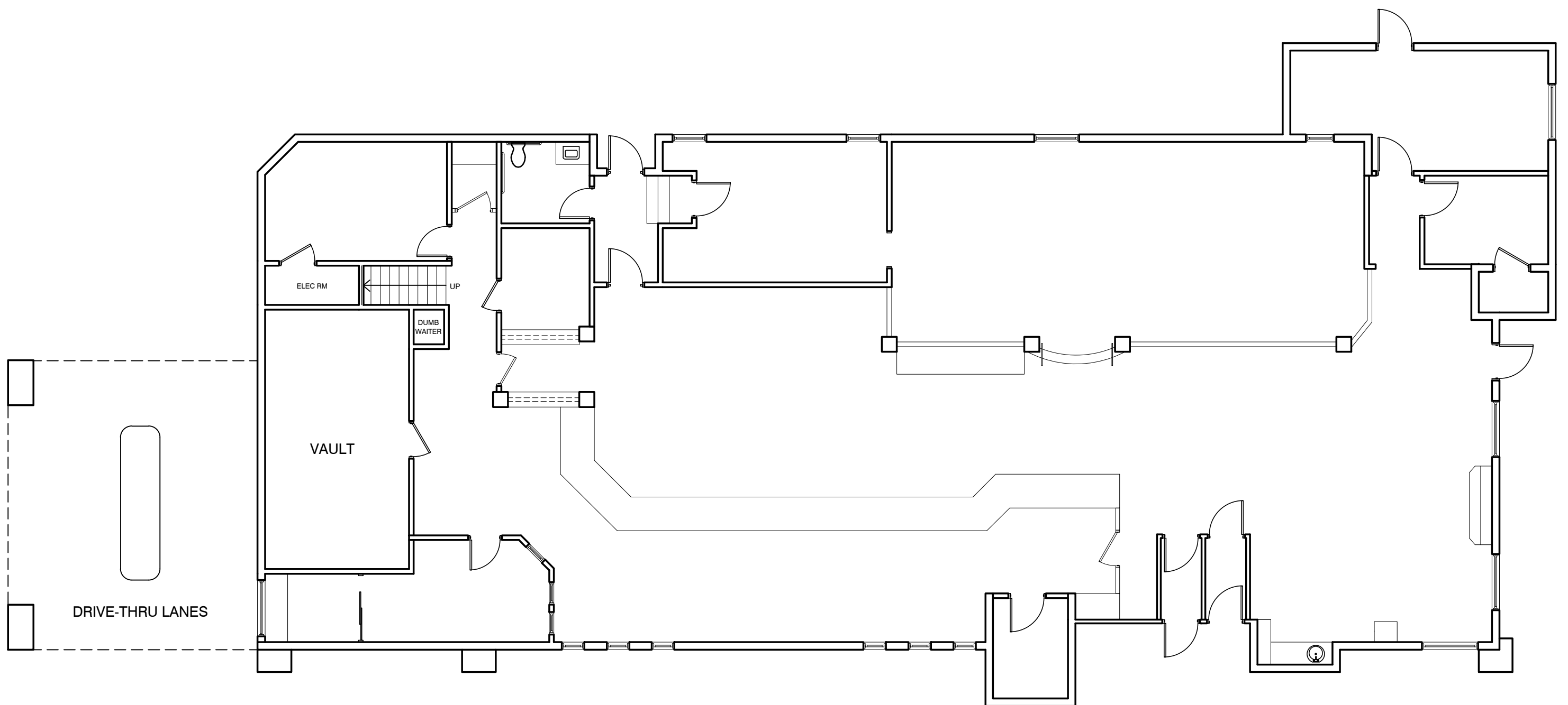
1ST FLOOR - 5,335 SF
