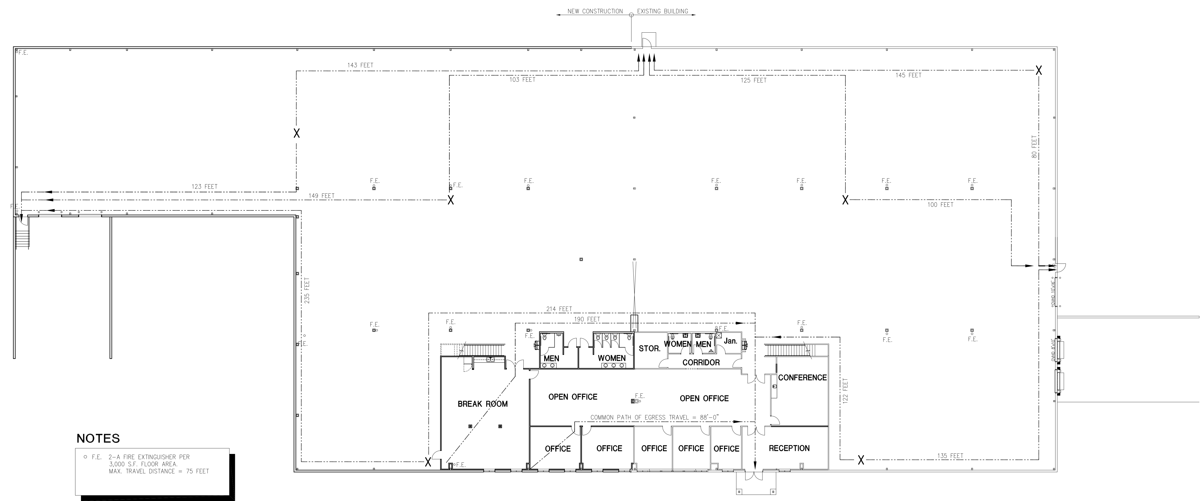
B MEZZANINE LIFE SAFETY PLAN A-0.1 SCALE: 3/32" = 1'-0"
