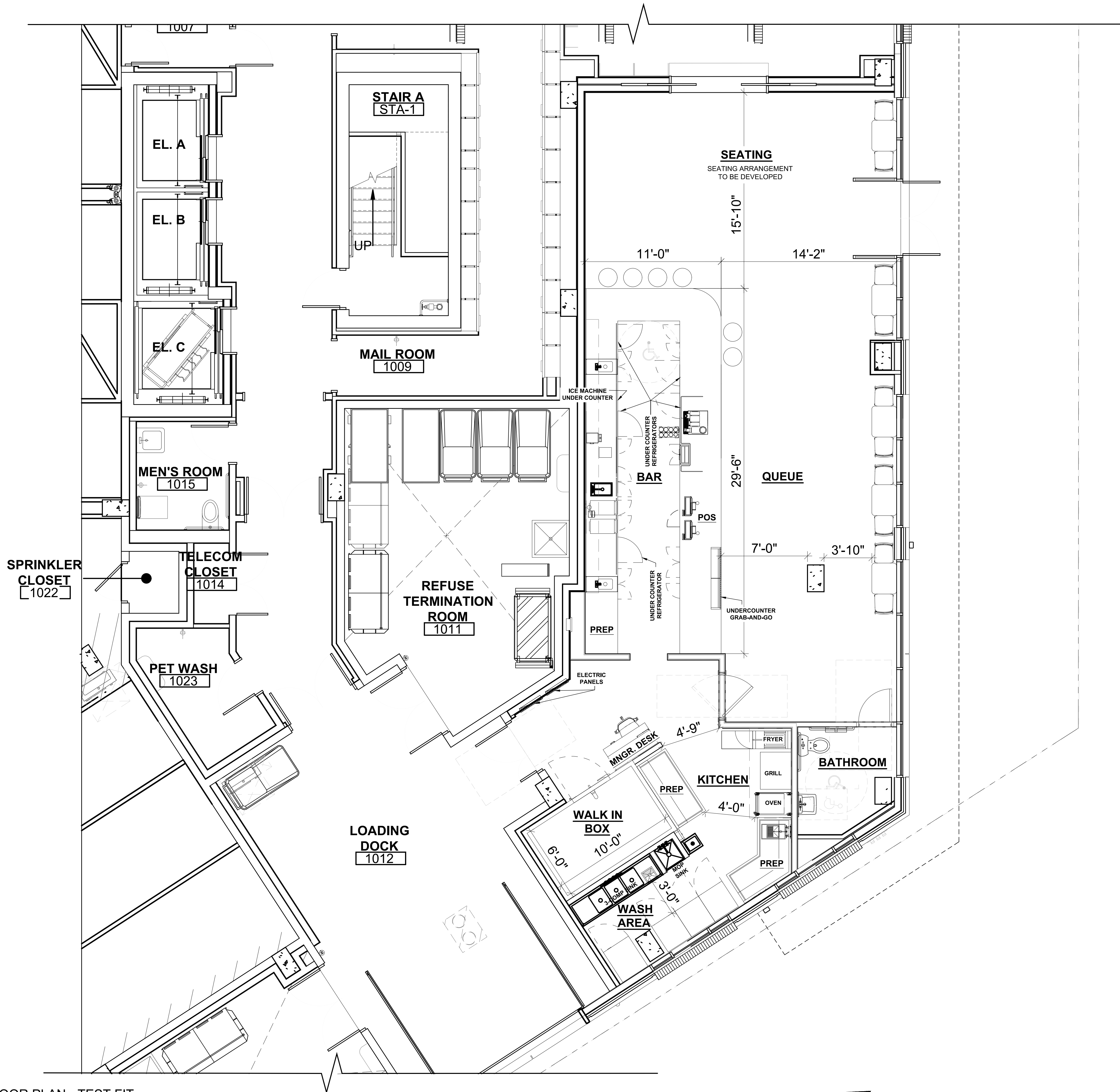
1 FIRST FLOOR PLAN - TEST FIT SCALE 1/4" = 1' - 0" 0 2' 4' 8' Scale: 1/4" = 1'-0"
