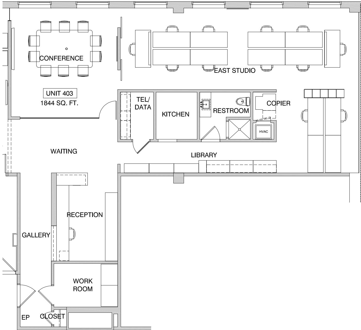
03 UNIT 403 FLOOR PLAN SCALE: 1/8"=1'-0"
