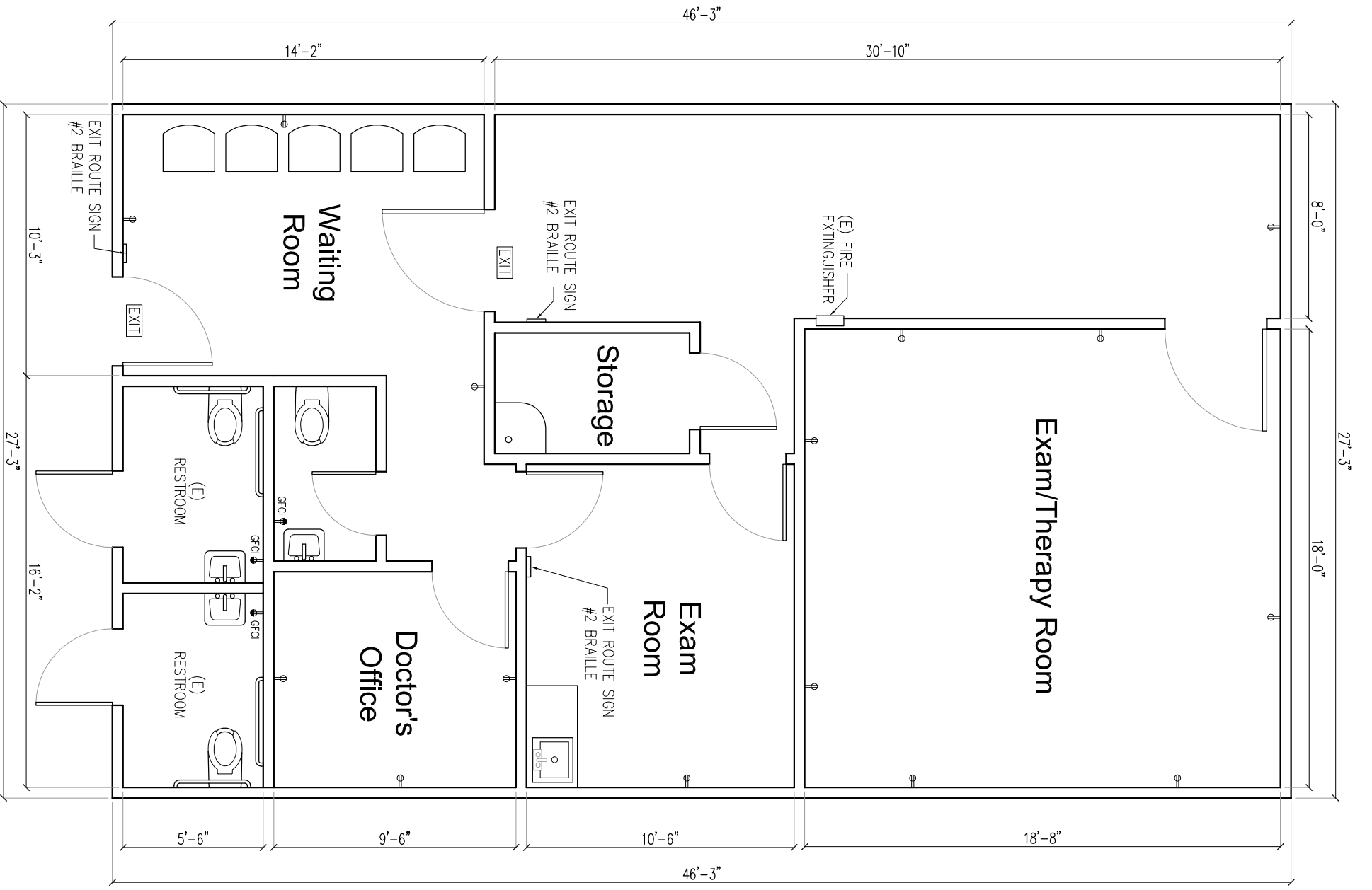
EXISTING FLOOR PLAN (SCALE:3/16"=1'-0")
