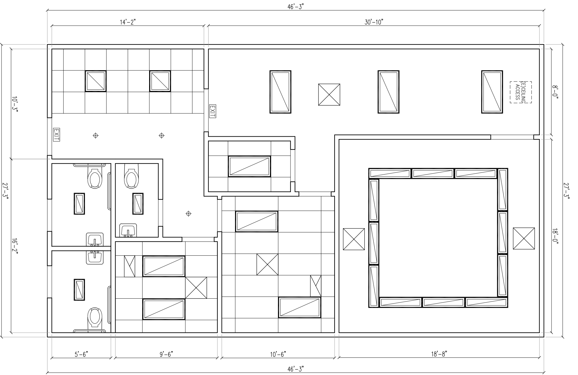
EXISTING CEILING PLAN (SCALE:3/16"=1'-0")
