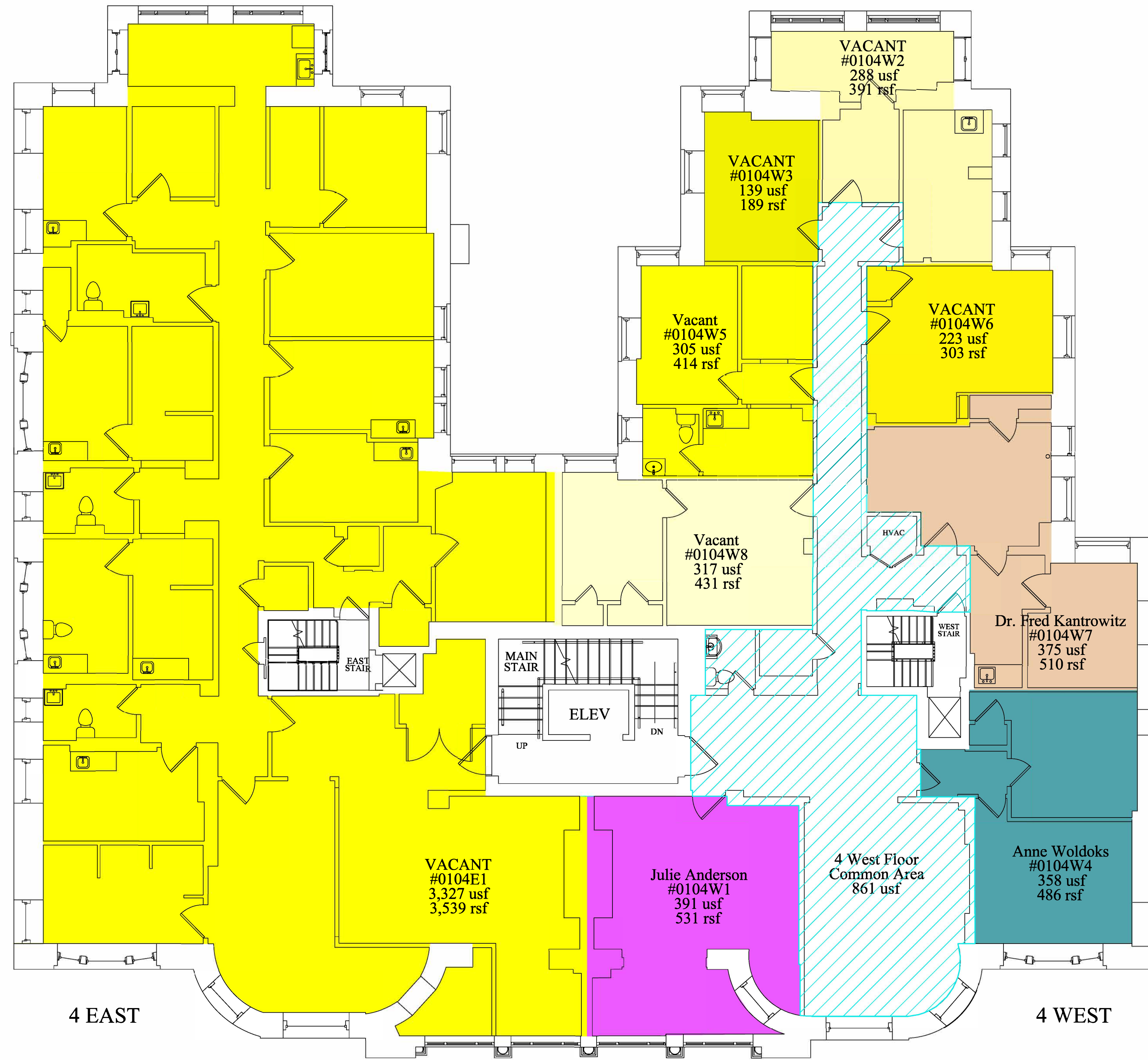
1 Fourth Floor Plan 3/16" = 1'-0"
