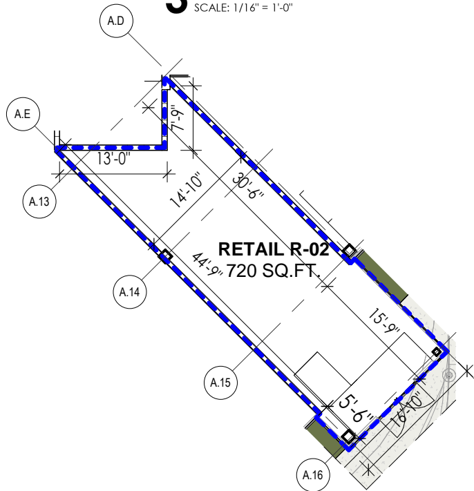
2 RETAIL SPACE - R02 LOD SCALE: 1/16" = 1'-0"
