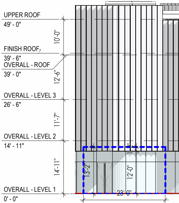
3 NORTH ELEVATION - RETAIL R02 SCALE: 1/16" = 1'-0"
