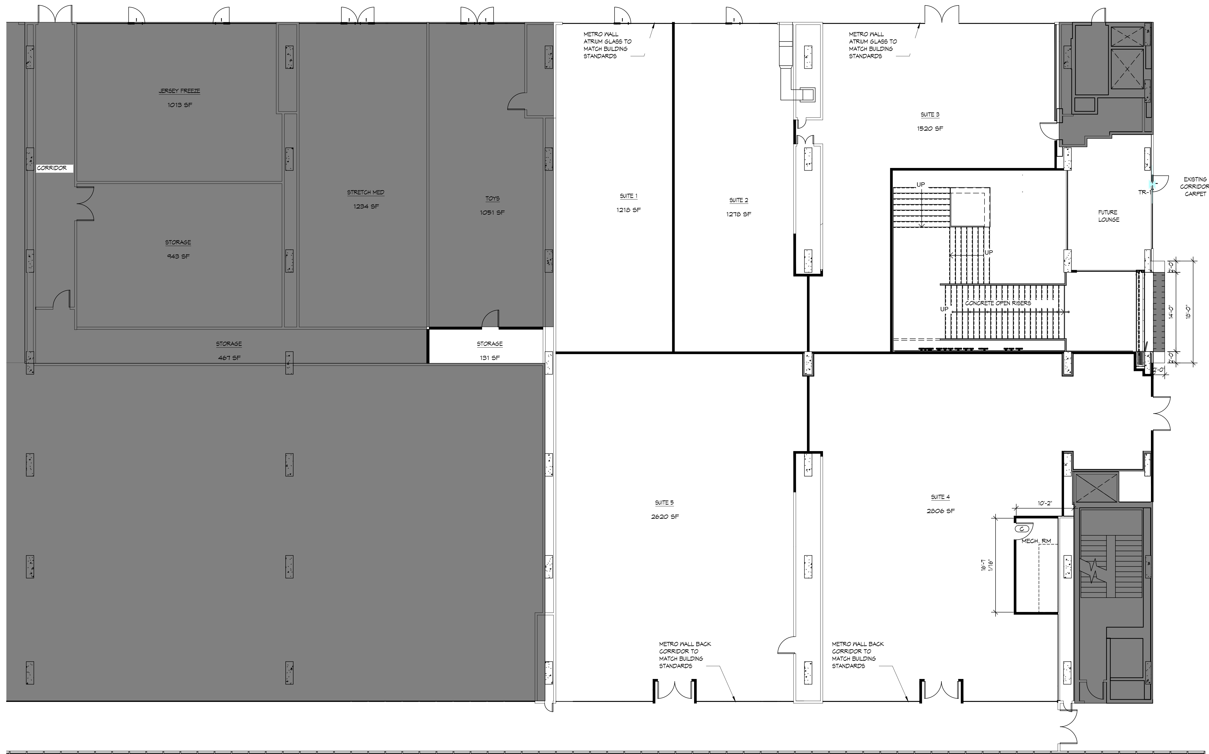
FIRST FLOOR - RETAIL SPACE PLAN SCALE: 1/8" = 1'-0"
