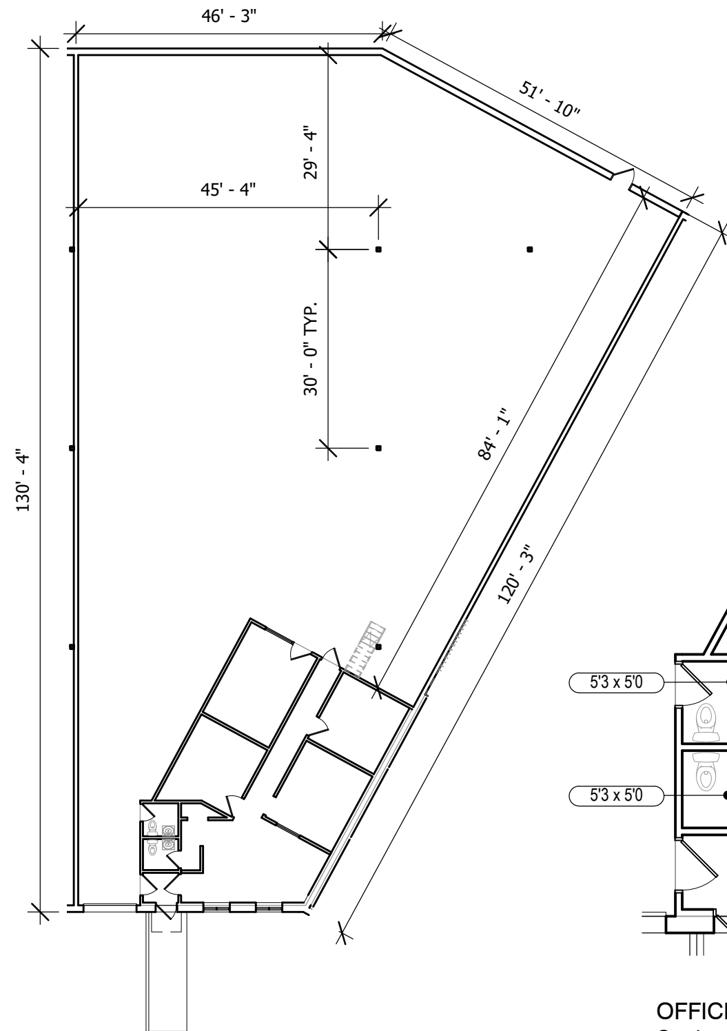
SUITE PLAN Scale: 1/20" = 1'-0"
