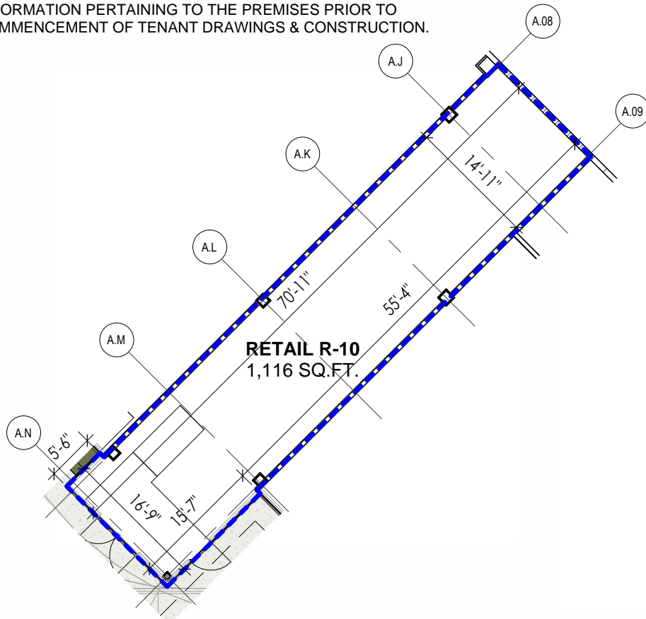
2 RETAIL SPACE - R10 LOD SCALE: 1/16" = 1'-0"
