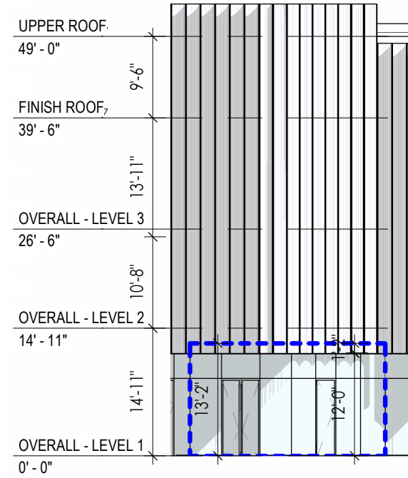
3 EAST ELEVATION- RETAIL R10 SCALE: 1/16" = 1'-0"
