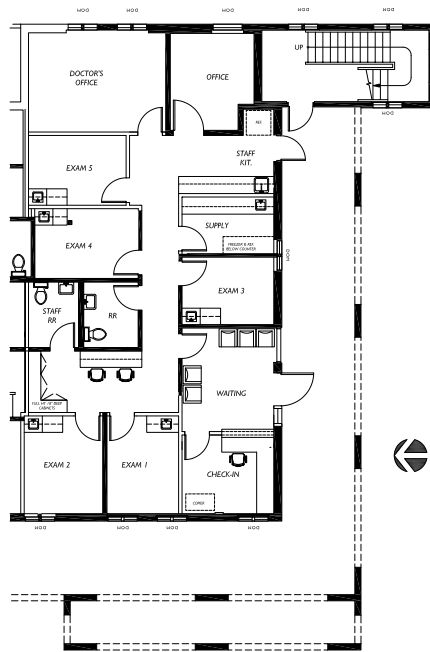
TEST-FIT PLAN
