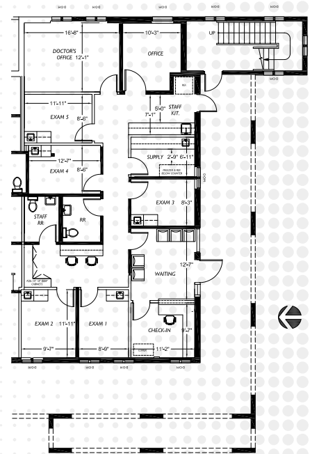
TEST-FIT PLAN (DIMENSIONS)
