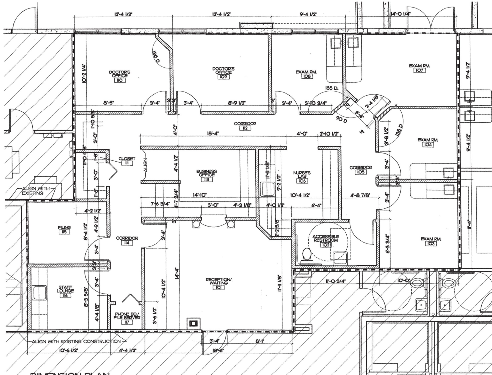
DIMENSION PLAN SCALE: 1/4" = 1'-0"
