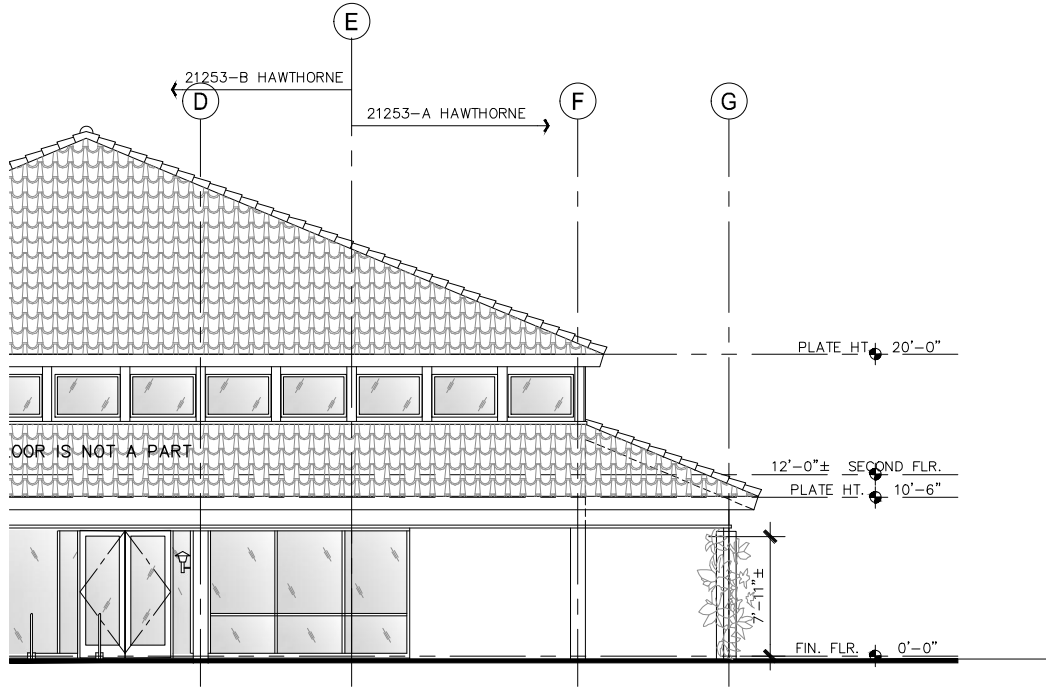
NORTH ELEVATION
