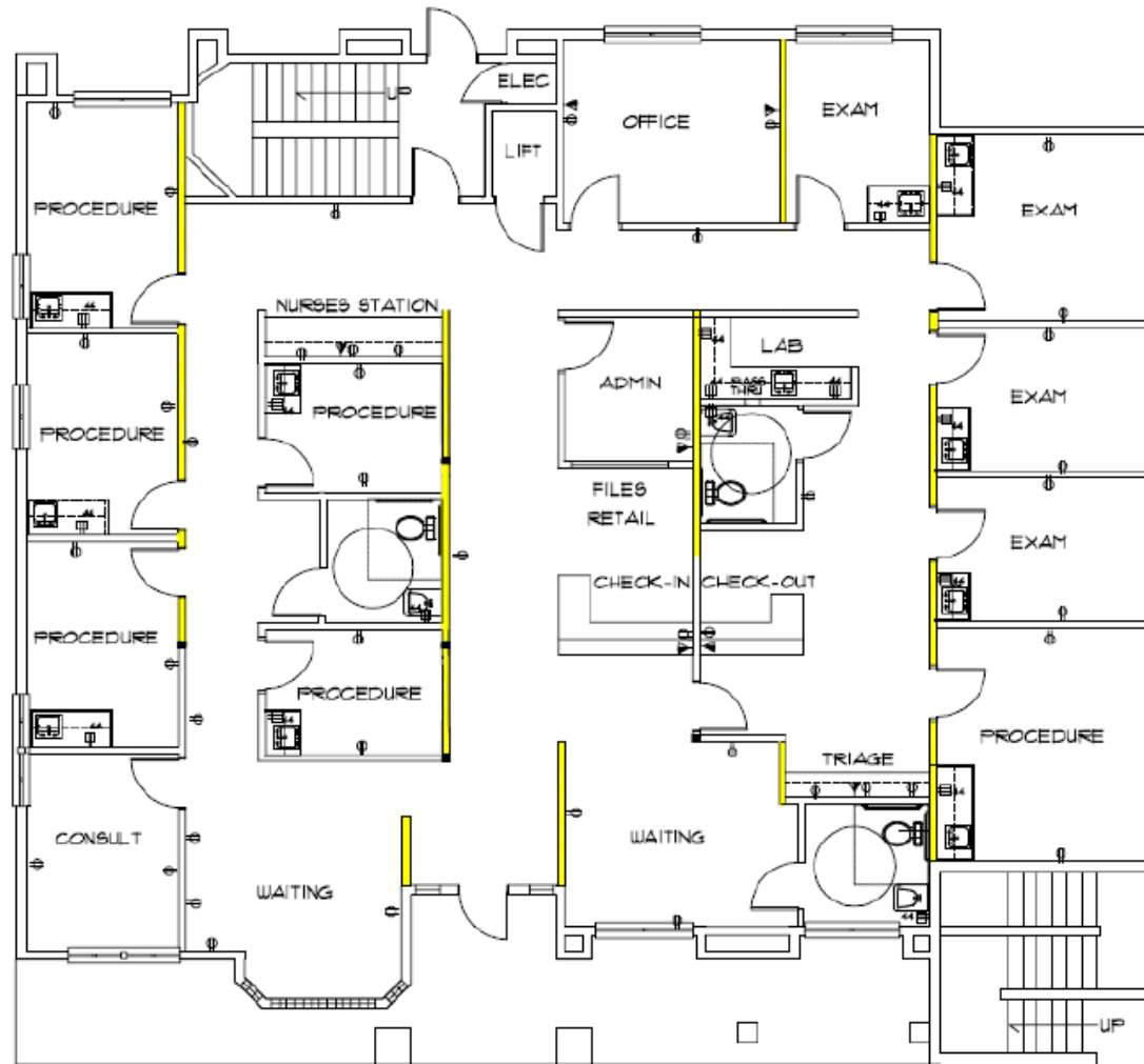
FIRST FLOOR ELECTRICAL PLAN
