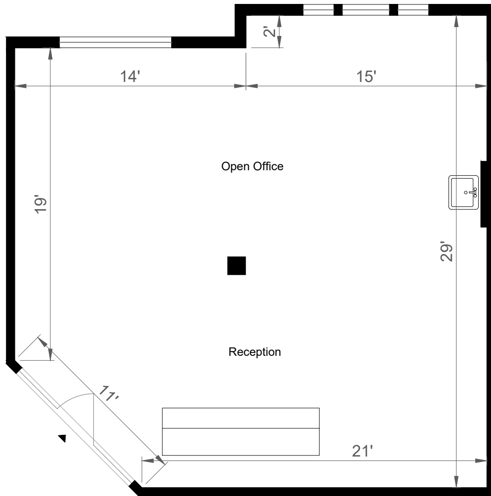
FLOOR PLAN
