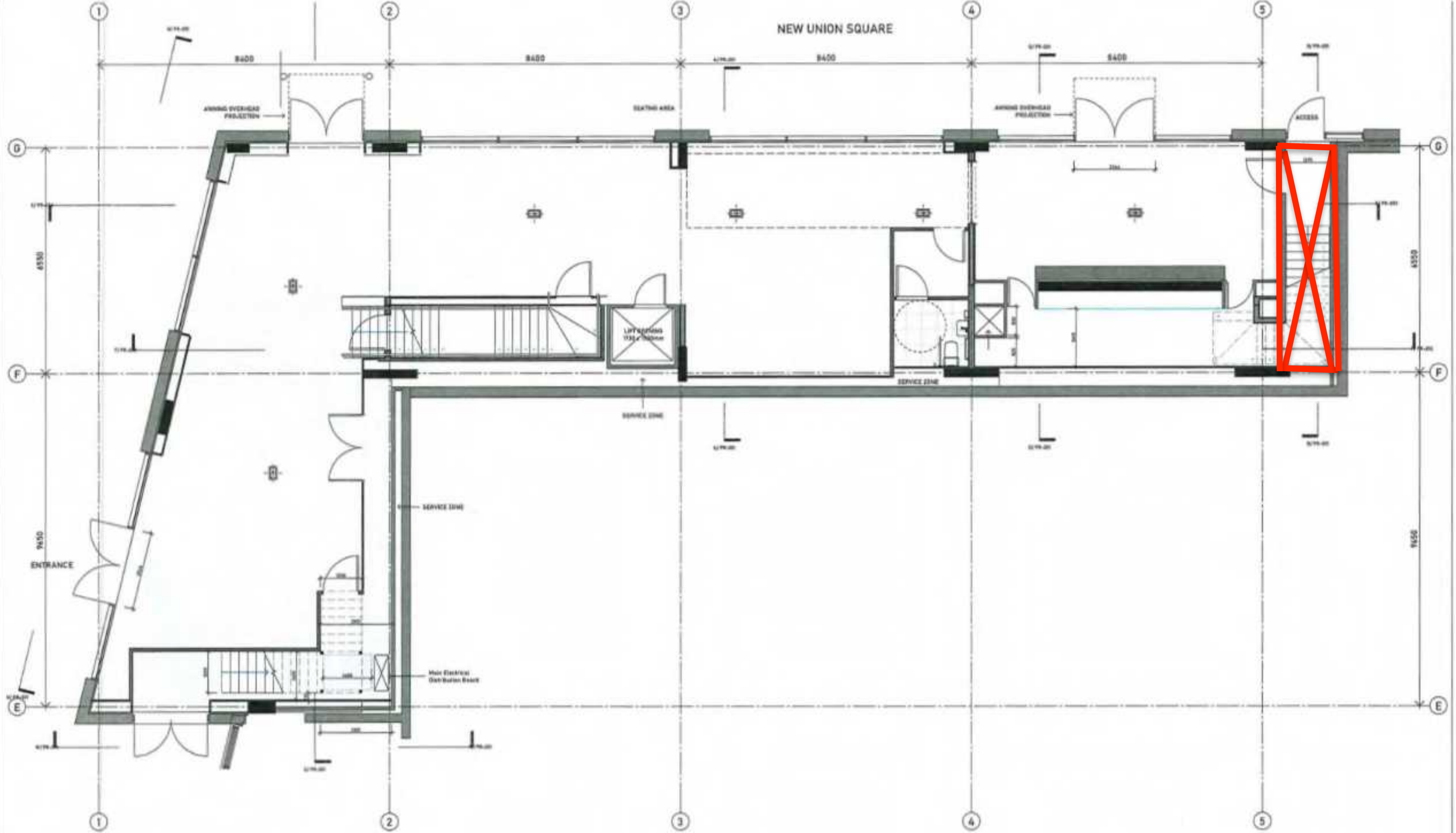
GA PLAN - LEVEL 0F
