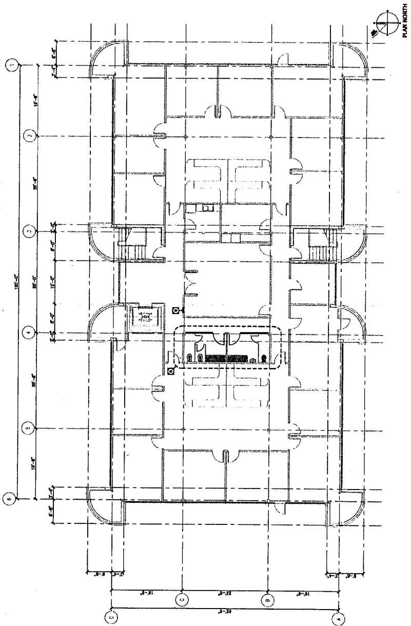
Floor Plan Suite 200
