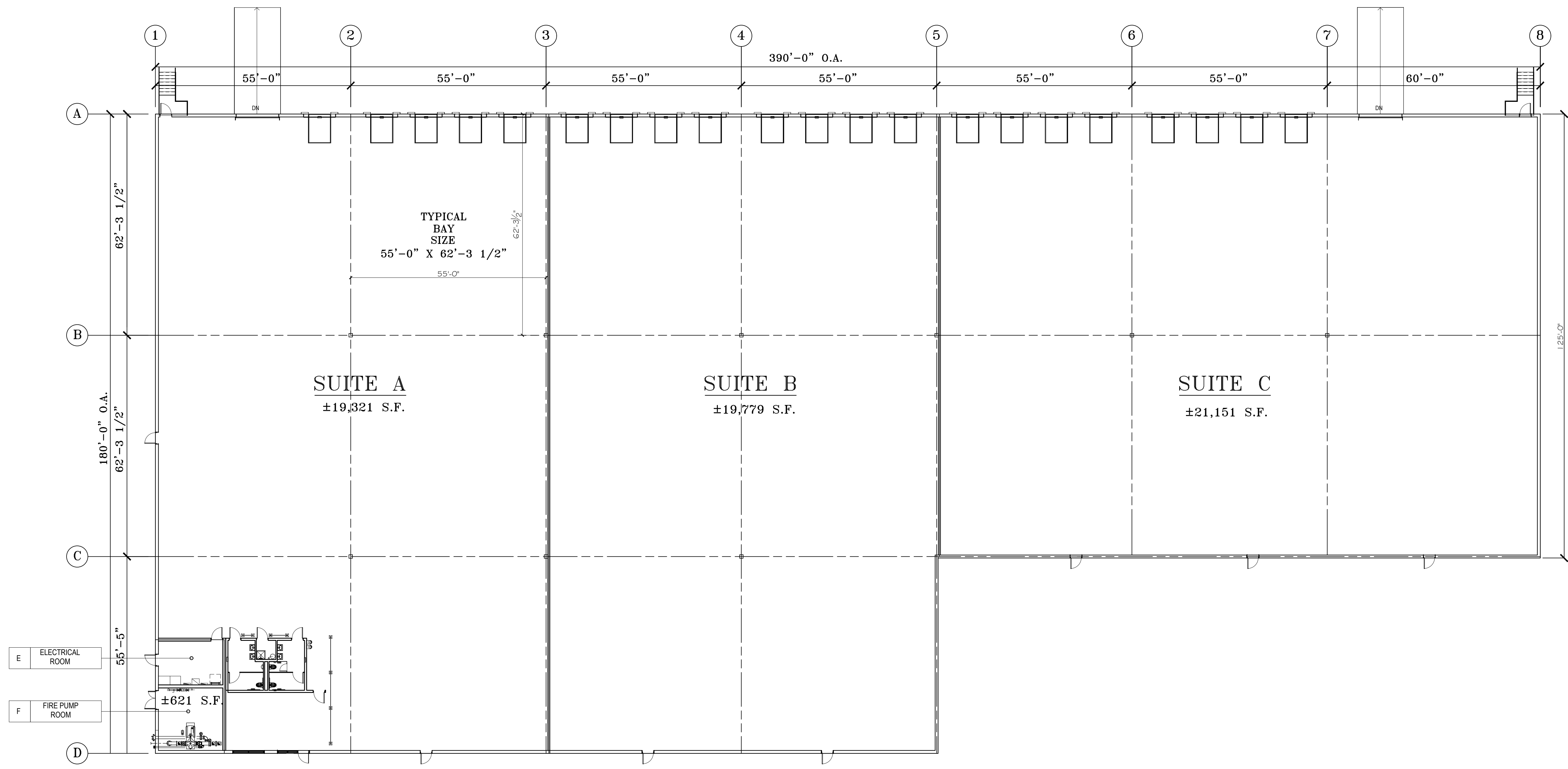
FLOOR PLAN SCALE: 1/16" = 1'-0" ±60,872 S.F.
