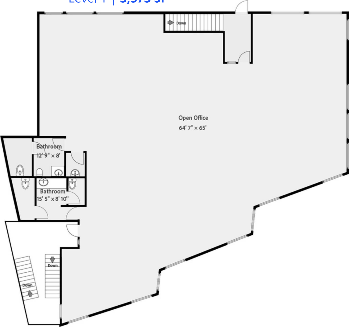
Level 1 | 3,373 SF
