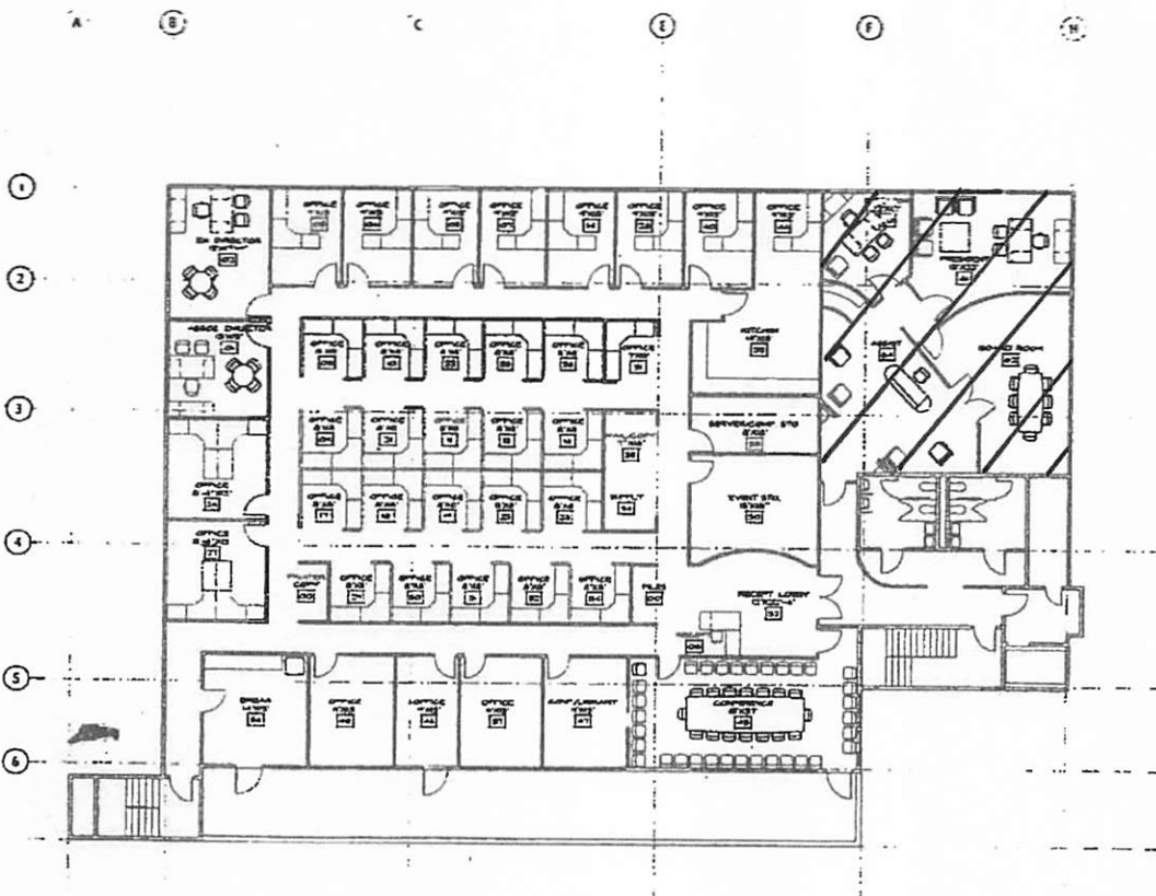
SECOND FLOOR PLAN 10/10/17 north
