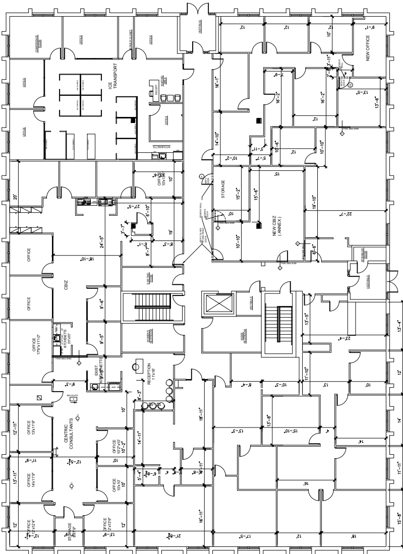
NEW INTERIOR LAYOUT SCALE: 1/8"=1'-0"
