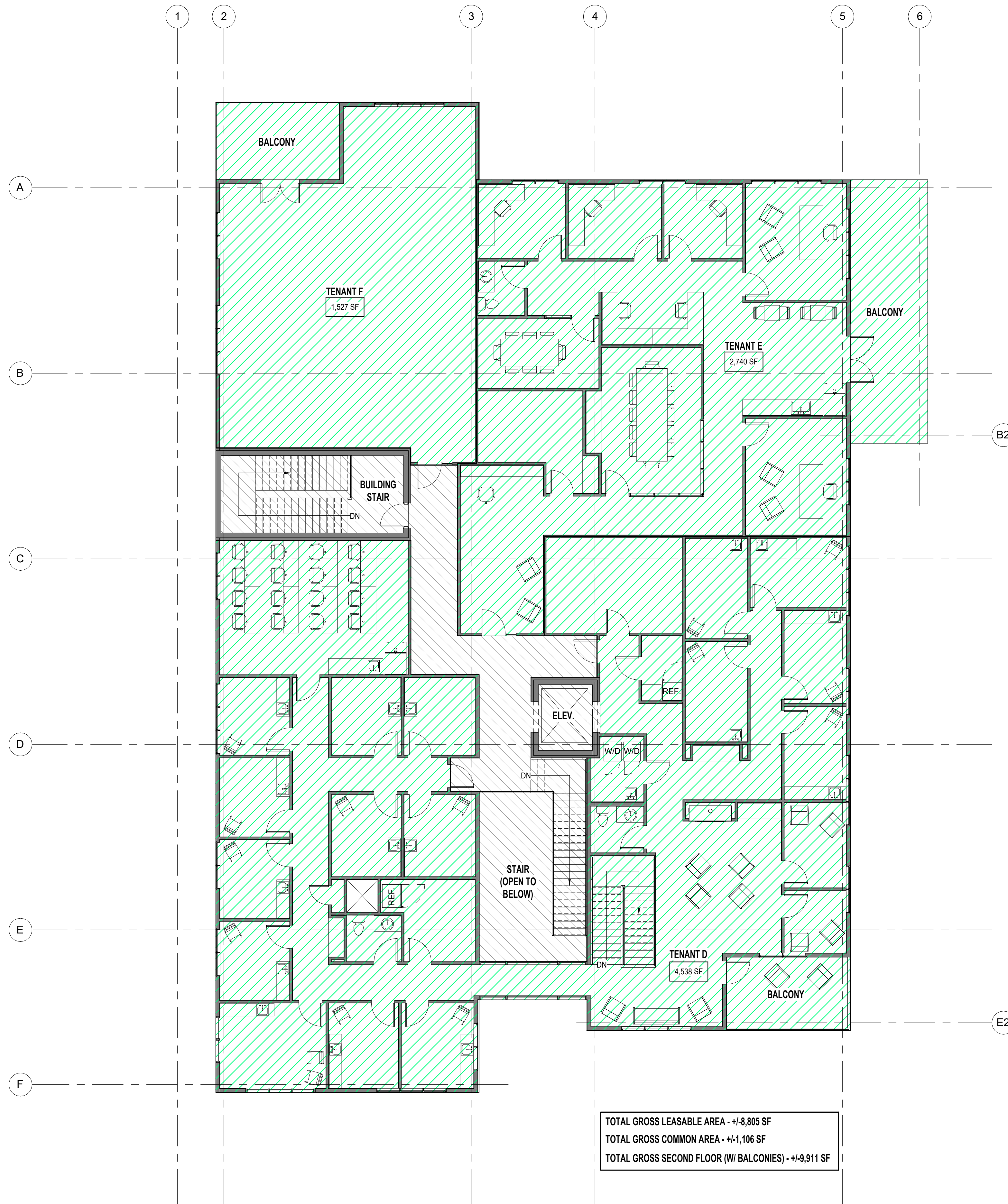
AREA PLAN - SECOND FLOOR SCALE: 1/8" = 1'-0"
