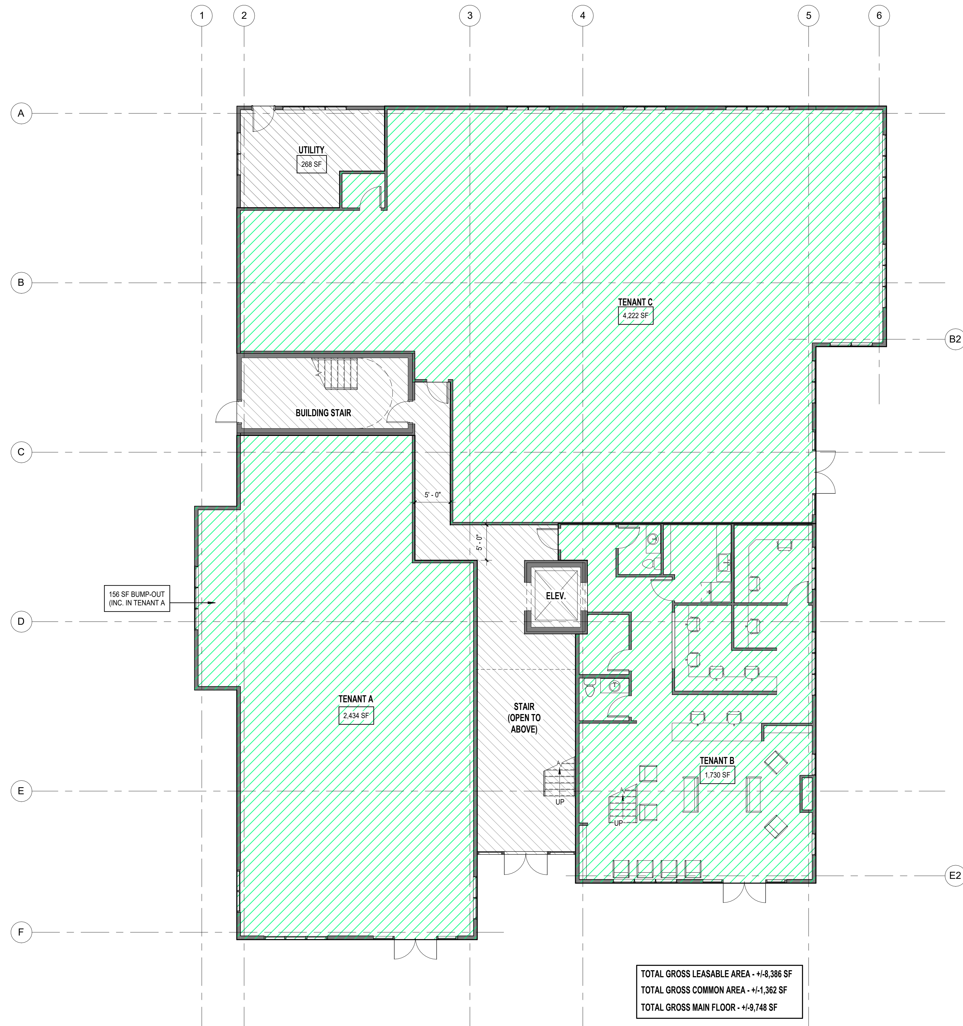
AREA PLAN - GROUND FLOOR SCALE: 1/8" = 1'-0"
