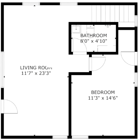
FLOOR 2
