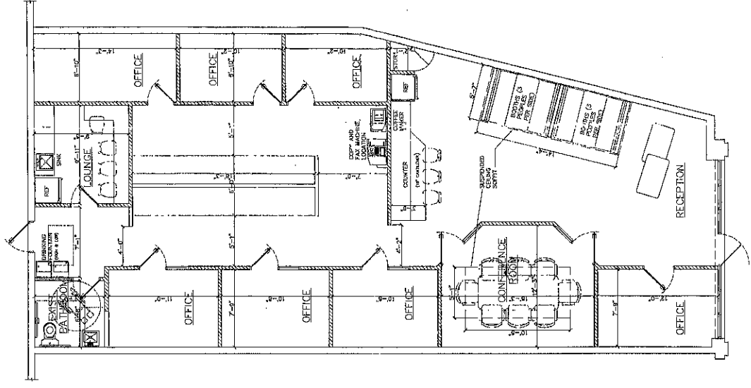
1 PROPOSED INTERIOR REMODELING FLOOR PLAN SCALE: AS SHOWN
