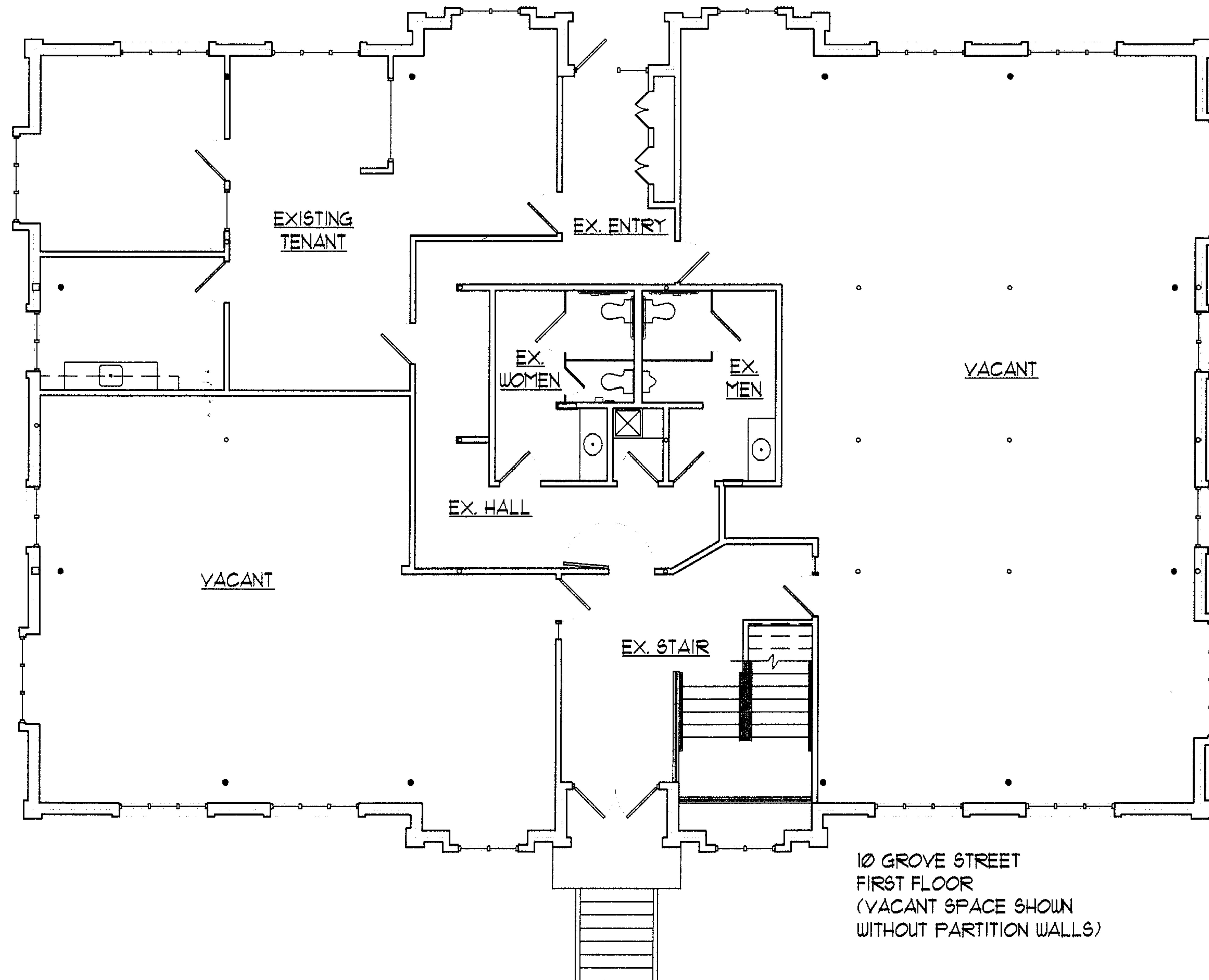
1 EXISTING FIRST FLOOR PLAN 3/32" = 1'-0"
