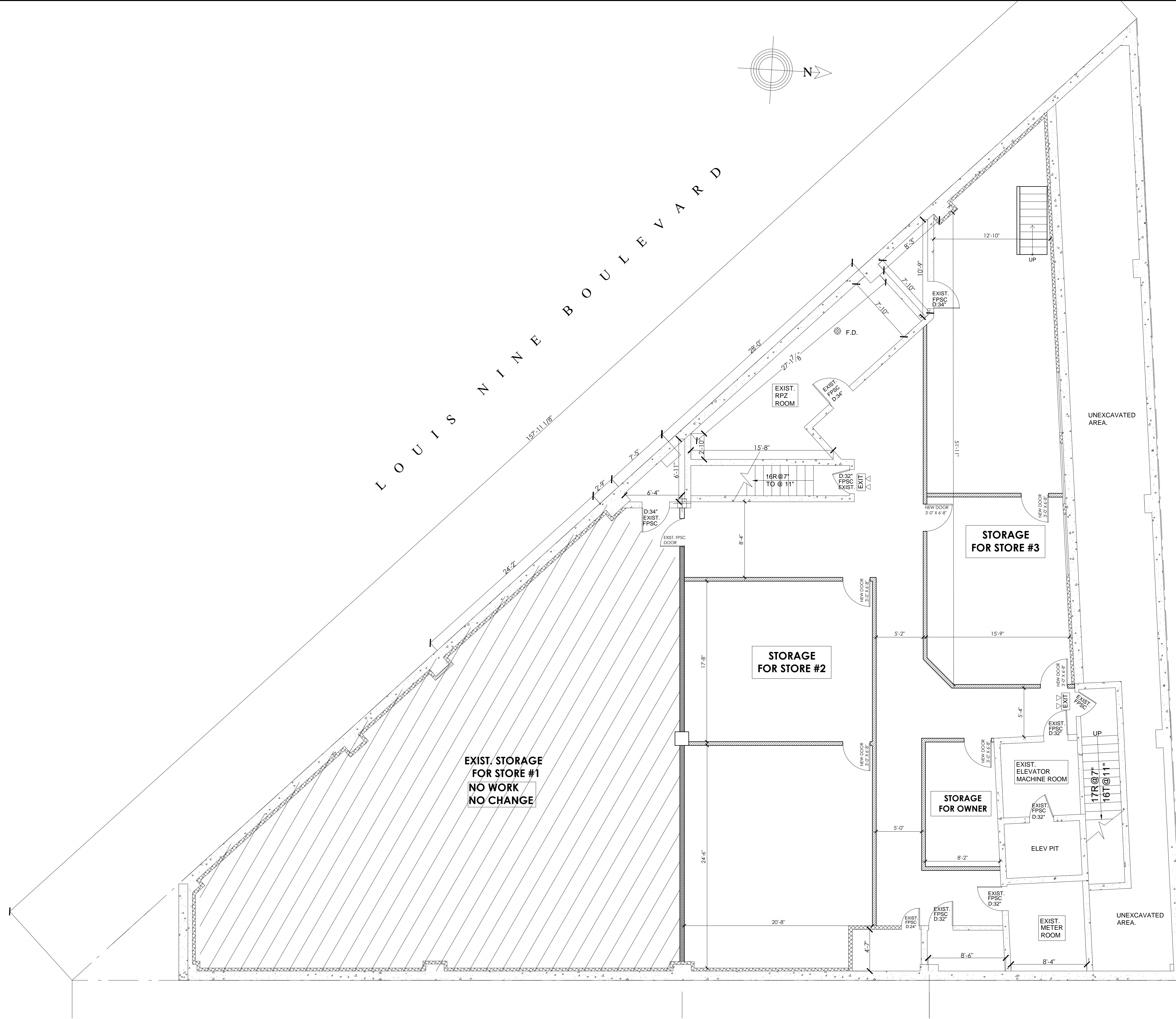
CELLAR PLAN SCALE: 3/16"=1'-0"
