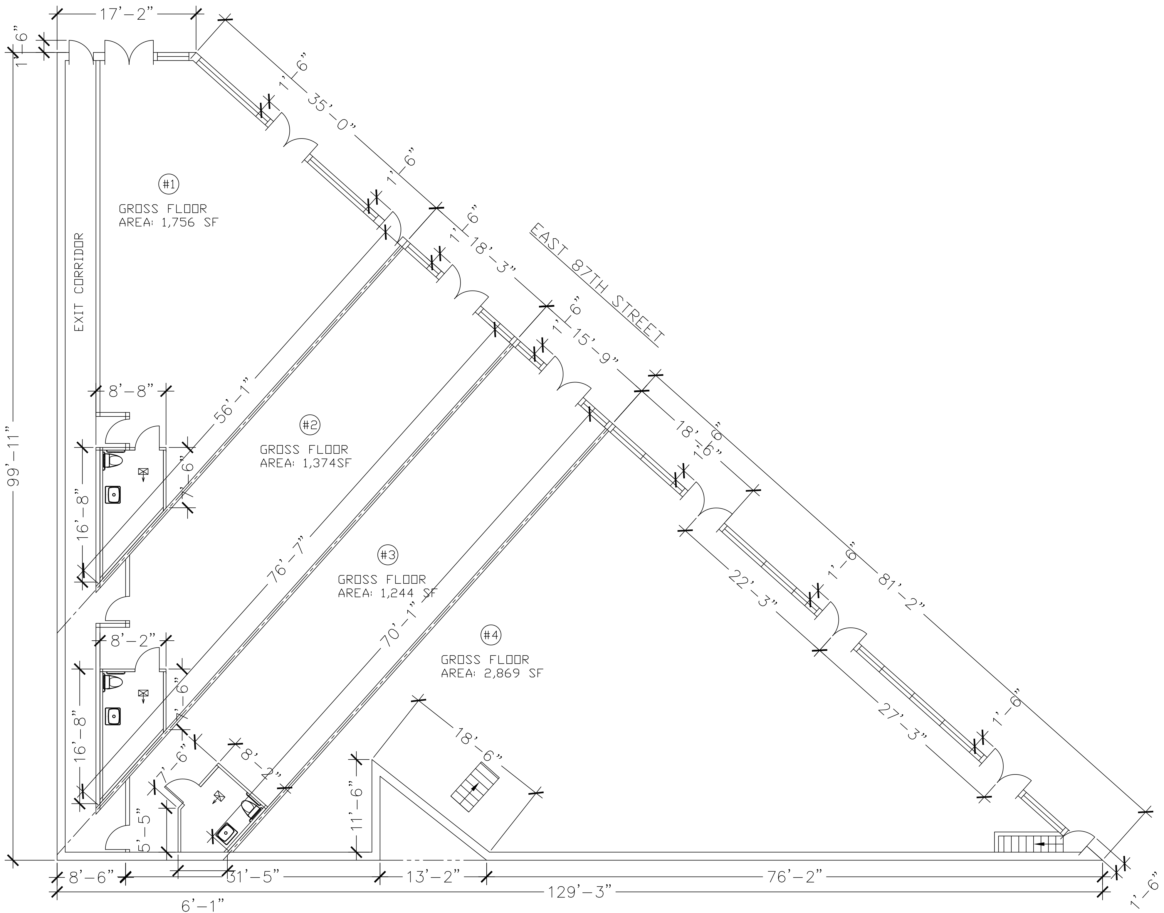
FIRST FLOOR PLAN SCALE: NTS
