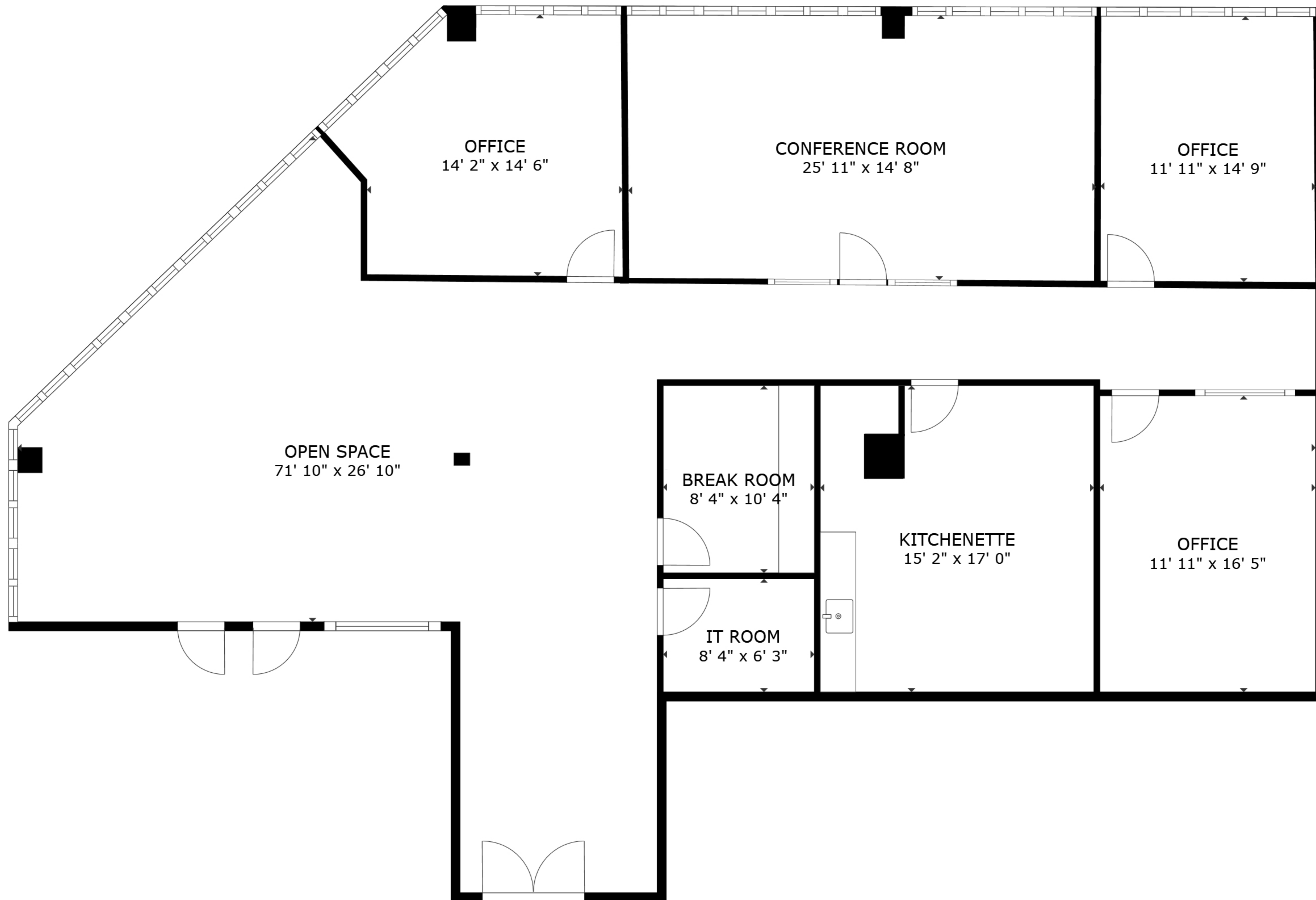
FLOOR PLAN
